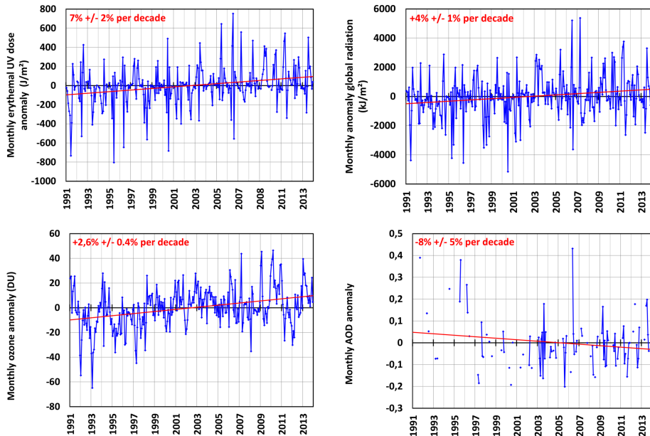
Fig. 2. Trends of monthly anomalies at Uccle for erythemal UV dose (upper left panel), global solar radiation (upper right panel), total ozone column (lower left panel) and AOD Aerosol Optical Depth at 320.1 nm (lower right panel) for the time period 1991-2013. The blue lines represent the time series, whereas the red lines represent the trend over the time period.
