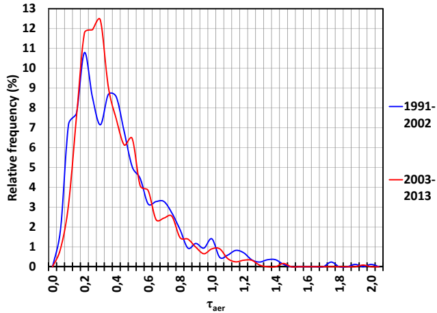
Fig. 4. Relative frequency distribution of daily AOD-Aerosol Optical Depth values for the two time periods: 1991-2002 (in blue) and 2003-2013 (in red).
