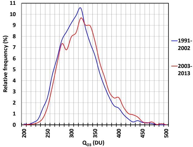
Fig. 3. Relative frequency distribution of daily TOC total ozone column values for the two time periods: 1991-2002 (in blue) and 2003-2013 (in red).
