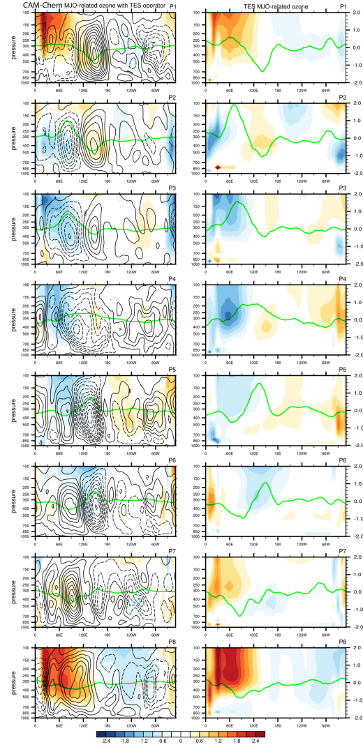
Fig. 6. Left: MJO-related ozone (color shades) for CAM-chem (with the TES operator applied) with GEOS-5 vertical velocity (black lines, dashed as negative and solid as positive) and precipitation (green lines, in m/s); Right: MJO-related ozone (color shades) for TES (color shades) with TRMM precipitation (green lines, in m/s).
