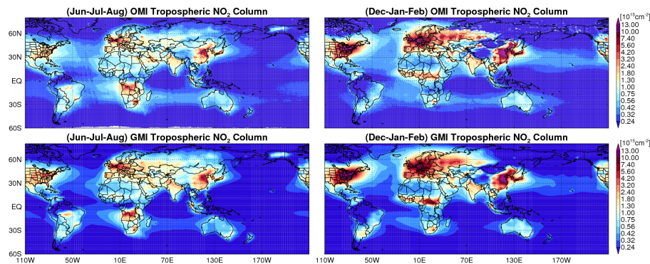
Fig. C3. For June–August (left column) and December–February (right column) averages over 2005–2007; top: OMI tropospheric column NO 2 ; bottom: GMI tropospheric column NO 2 .
