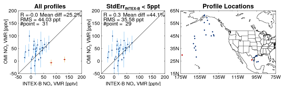
Fig. 3. Scattergram of INTEX-B and OMI cloud slicing NO 2 VMRs; left: all available collocations of INTEX-B and OMI NO 2 VMR; middle: collocations where the INTEX-B standard error of the mean < 5 pptv; right: locations of the profiles. Red shows cases where the INTEX-B standard error of the mean > 5 pptv.
