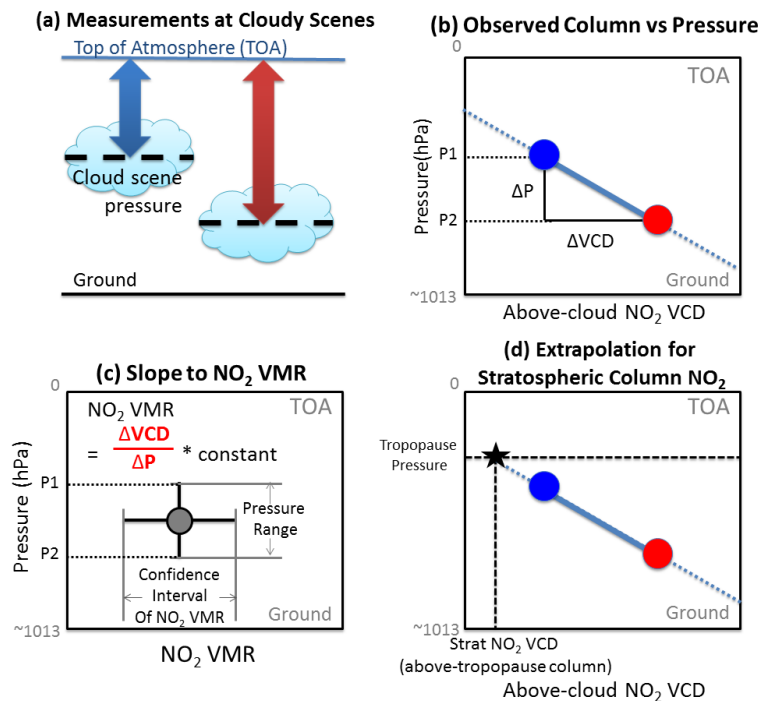
Fig. 1. Schematic view of the cloud slicing technique (not to scale): (a) two above-cloud \text{NO}_2 column measurements at different cloud scene pressures (blue: column with lower scene pressure; and red: column with higher scene pressure); (b) the measurements shown on a pressure-column coordinate plane; (c) \text{NO}_2 VMR derived from the slope of above-cloud \text{NO}_2 VCD vs. cloud scene pressure with confidence interval (horizontal error bar) and pressure range (vertical error bar); (d) stratospheric column \text{NO}_2 derived by extrapolating the linear fit to the tropopause.
