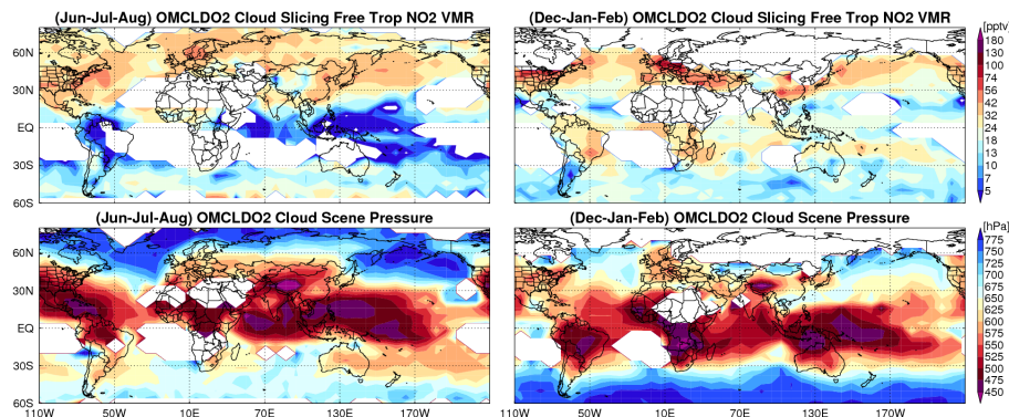
Fig. D2. For June–August (left) and December–February (right) averaged over 2005–2007, top: global maps of NO 2 VMR calculated using OMCLDO2 cloud parameters; bottom: mean cloud scene pressures from OMCLDO2.
