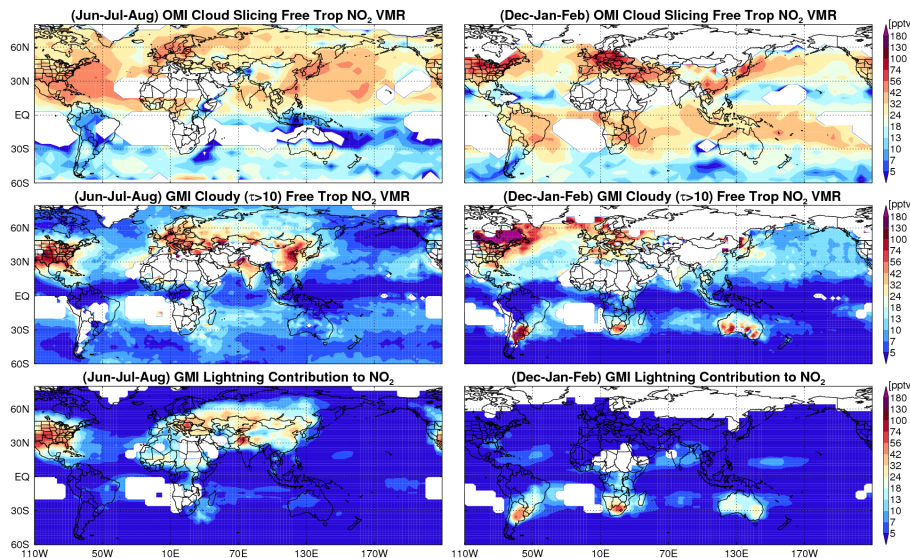
Fig. 4. For June–August (left column) and December–February (right column) averages over 2005–2007; first row: climatology of free tropospheric NO 2 VMR; second row: cloudy ( \tau > 10 ) GMI free tropospheric NO 2 VMR; third row: GMI lightning contribution to the free tropospheric NO 2 VMRs.
