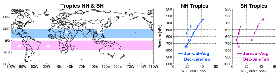
Fig. 6. Left: sampling areas for profiles over tropics of NH (blue) and SH (purple); center: NO 2 profiles over NH tropics for June–August (blue solid line) and December–February (blue dotted line) with standard errors; right: NO 2 profiles over SH tropics for June–August (purple solid line) and December–February (purple dotted line) for 2005–2007.
