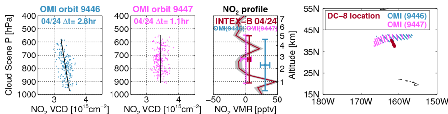
Fig. B3. Similar to Fig. 2, but showing an example of variation in OMI NO 2 VMRs over two adjacent orbits (1.5 h time difference) at the same location north of Hawaii, US.
