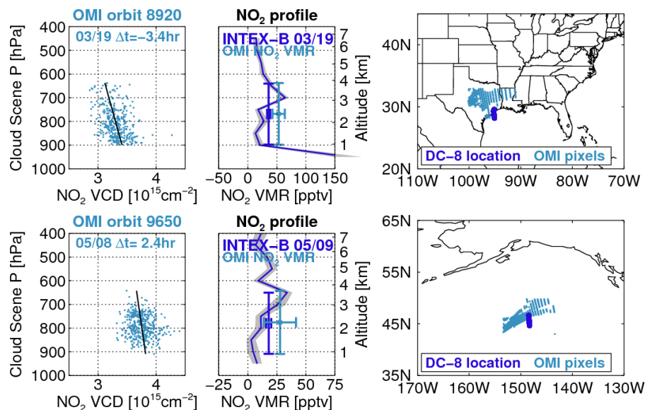
Fig. 2. Examples of relatively good agreement between OMI cloud slicing VMRs and INTEX-B NO 2 profiles near Houston, Texas, US (top row) and the northeastern Pacific (bottom row). In each example, left: OMI above-cloud NO 2 column vs. cloud scene pressure (similar to Fig. 1b); center: INTEX-B NO 2 profiles (dark blue line), INTEX-B NO 2 VMR averaged over the OMI pressure range (dark blue square with error bars), and OMI-derived NO 2 VMR (light blue square with error bars); right: locations of OMI and INTEX-B aircraft measurements.
