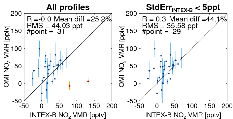
Fig. D1. Similar to Fig. 6 but using geometric AMF.
