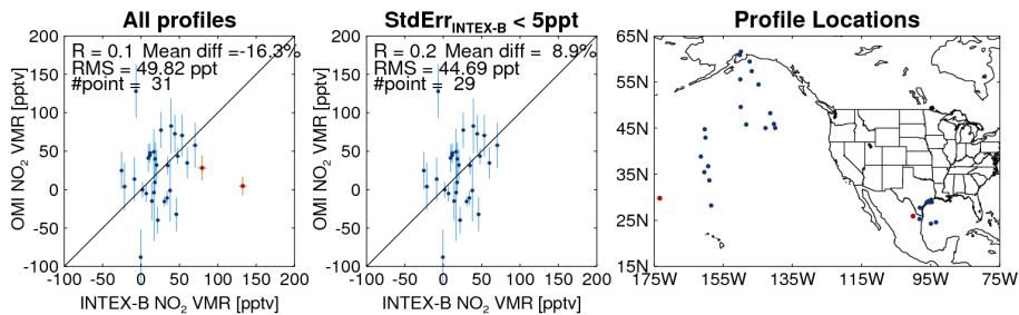
Fig. 6. Scattergram of INTEX-B and OMI cloud slicing \text{NO}_2 VMRs; left: all available collocations of INTEX-B and OMI \text{NO}_2 VMR; middle: collocations where the INTEX-B standard error of the mean < 5 pptv; right: locations of the profiles. Red shows cases where the INTEX-B standard error of the mean > 5 pptv.
