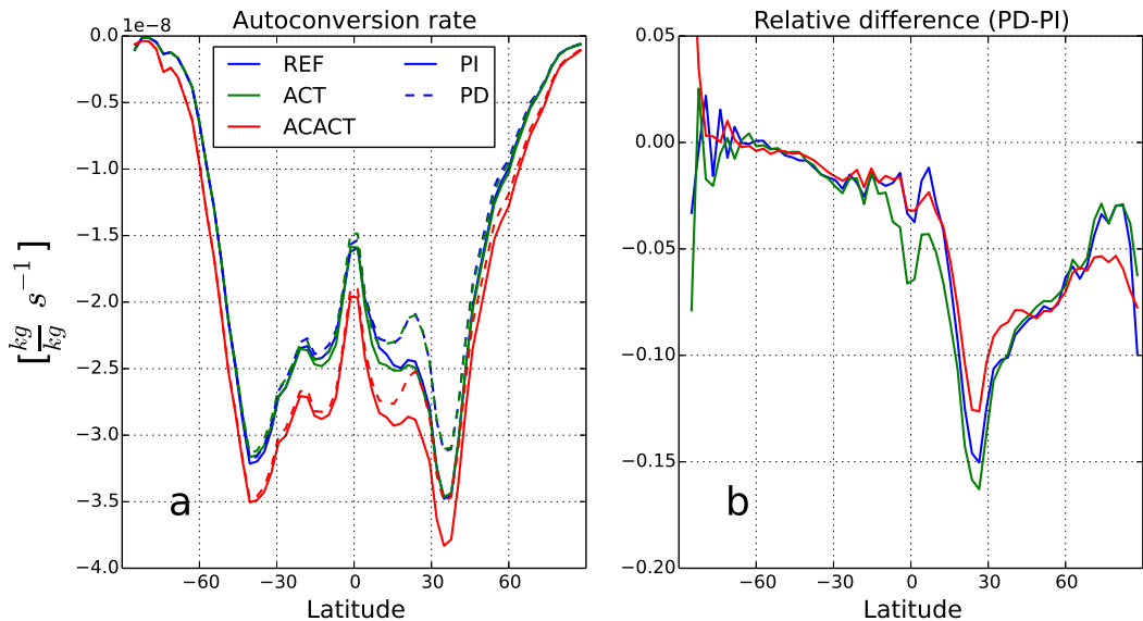
Fig. 2. (a) Autoconversion rate for PI and PD conditions in \text{s}^{-1} at 890 hPa and (b) the relative anthropogenic change for each model configuration.
