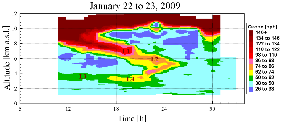
Figure 11. Ozone soundings on 22 and 23 January 2009; four intrusion layers (L1, L2, L3, L4) have been identified, corresponding to different advection pathways (see text).
