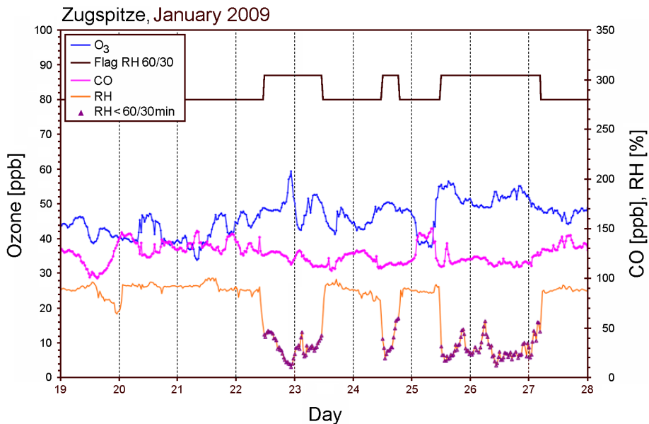
Figure 13. Zugspitze data around 22 January 2009; the maximum of intrusion layer L4 is visible during the final hours of 22 January. CO drops by only 10 ppb during that period.
