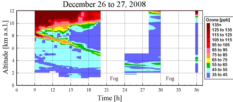
Figure 6. Time series of ozone from lidar measurements on 26 and 27 December 2008, showing a very thin stratospheric air intrusion descending from the tropopause to almost 3 km a.s.l.; after the descent the intrusion seems to climb again to more than 4 km.
