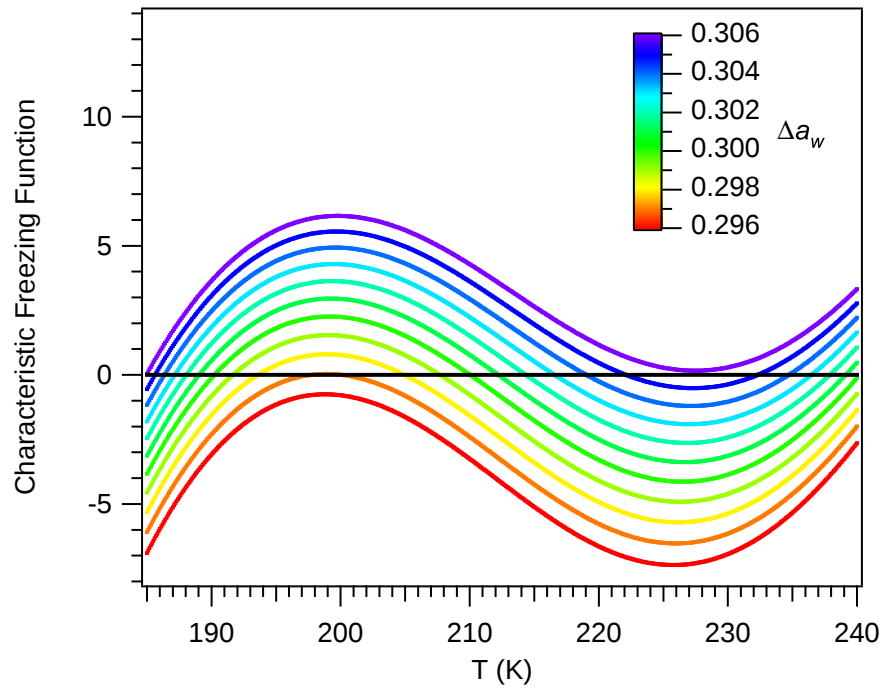
Fig. 7. Characteristic freezing function for D_p = 10 \mu\text{m} and \Delta t = 10 \text{ s} .
