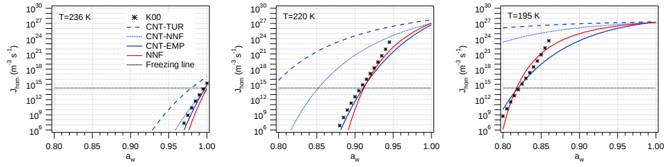
Fig. 4. Homogeneous nucleation rate. K00 and NNF correspond to J_{\text{hom}} obtained using the correlations of Koop et al. (2000) and the NNF model (Eq. 19) respectively. For CNT \sigma_{\text{iw}} was calculated using the Turnbull (1950) correlation (CNT-TUR, Eq. 25), an empirical correlation derived from fitting CNT to the K00 parameterization (CNT-EMP, Eq. 29), and a theoretical expression derived from the NNF model (CNT-NNF, Eq. 27).
