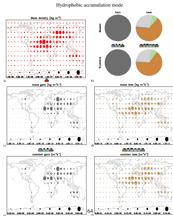
Figure 14. Global distribution of annual burdens (a) and tendencies (b–f) of the hydrophobic accumulation mode. The colours indicate either species (defined in Table 3) or processes (defined in Table 2). The pie-chart shows fractional contributions, while the radius of the pie indicates total column burden or total column tendency (logarithmic scale as shown in black at the bottom of panels a , c–f ). Panel (b) shows a global average of the tendencies.
