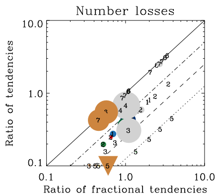
Figure 26. Pre-industrial (PI) to Present Day (PD) ratios of absolute tendencies against PI to PD ratios of fractional tendencies. Colours indicate processes (Table 2), numbers indicate modes (Table 3). The size of the symbol indicates fractional tendency in the PD experiment, with the largest symbols having a fractional tendency of about 1 (linear scale). The slanted lines represent y = 2^{-n}x , with n = 0, 1, 2, 3 . Results are shown for East Asia.
