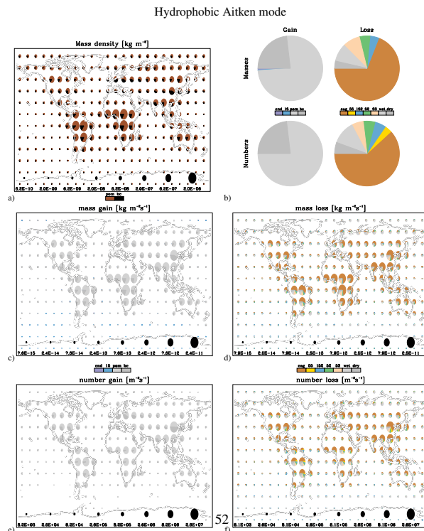
Figure 8. Global distribution of annual burdens (a) and tendencies (b–f) of the hydrophobic Aitken mode. The colours indicate either species (defined in Table 3) or processes (defined in Table 2). The pie-chart shows fractional contributions, while the radius of the pie indicates total column burden or total column tendency (logarithmic scale as shown in black at the bottom of panels a , c–f ). Panel (b) shows a global average of the tendencies.
