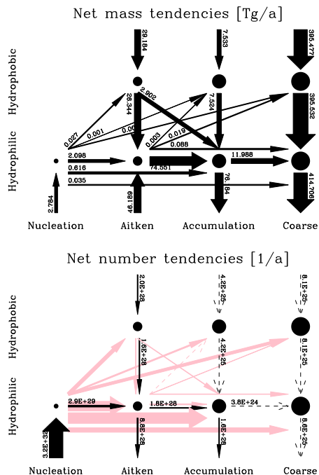
Figure 4. Globally and annually averaged net mass and number tendencies (arrows) between the 7 modes (dots) in ECHAM5.5-HAM2. The vertical arrows at the top and bottom of the figure represent H 2 SO 4 nucleation, condensation and production, aerosol primary emission and deposition processes. The arrows between the modes represent coagulation, ageing and redistribution processes. Pink arrows are number loss tendencies for coagulation processes. The width of the arrow scales logarithmically with the magnitude of the net tendency. In addition, numerical values for the annual and global averages are given.
