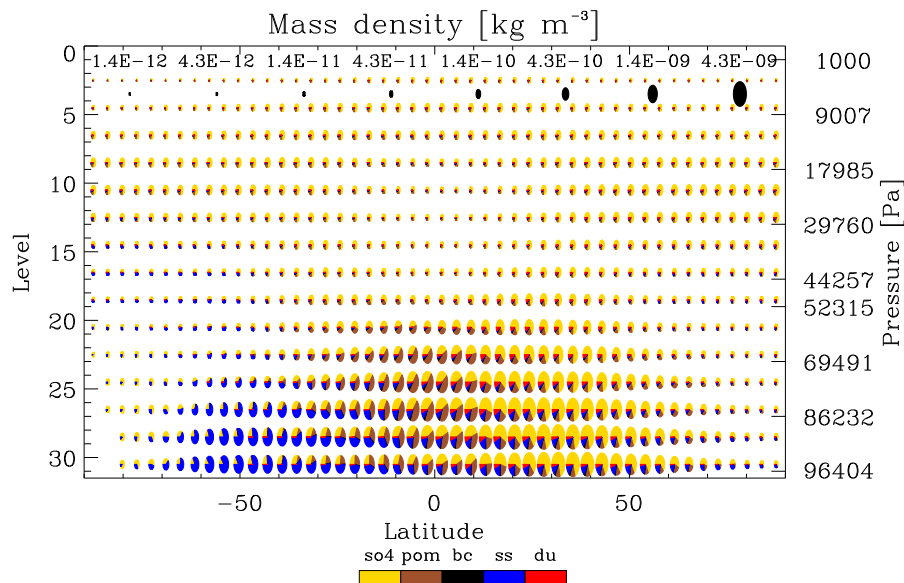
Figure 16. Zonal distribution of annual densities of the hydrophilic accumulation mode. The colours indicate species (defined in Table 3). The pie-chart shows fractional contributions, while the radius of the pie indicates the zonally-averaged density (logarithmic scale as shown in black at the top).
