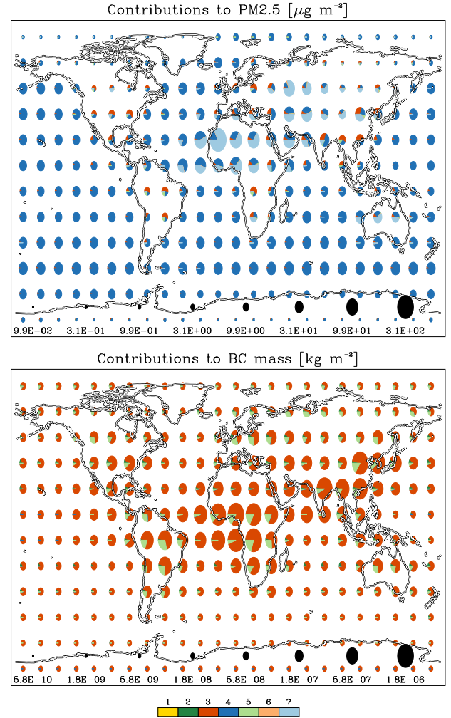
Fig. 3. Contributions by different modes to surface PM2.5 and black carbon mass burden for the baseline experiment. The pie-chart colours show contribution by mode (see legend below lowest panel), the pie-chart's size the overall magnitude (legend at the bottom of each panel). From top to bottom: surface PM2.5 (logarithmic scale); black carbon mass burden (logarithmic scale).
