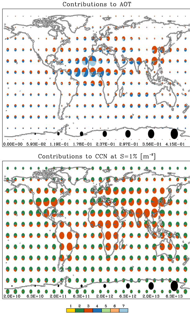
Fig. 2. Contributions by different modes to AOT and CCN for the baseline experiment. The pie-chart colours show contribution by mode (see legend below lowest panel), the pie-chart's size the overall magnitude (legend at the bottom of each panel). From top to bottom: AOT at 550nm (linear scale); column-integrated CCN at S=1% (logarithmic scale).
