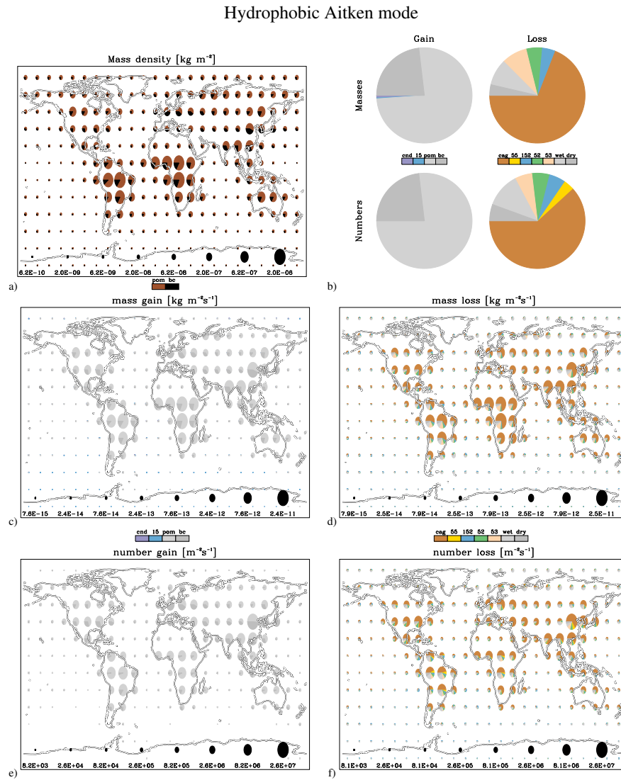
Fig. 8. Global distribution of annual burdens (a) and tendencies (b,c,d,e and f) of the hydrophobic Aitken mode. The colours indicate either species (defined in Table 3) or processes (defined in Table 2). The pie-chart shows fractional contributions, while the radius of the pie indicates total column burden or total column tendency (logarithmic scale as shown in black at the bottom of panels a,c,d,e and f). Panel b shows a global average of the tendencies.
