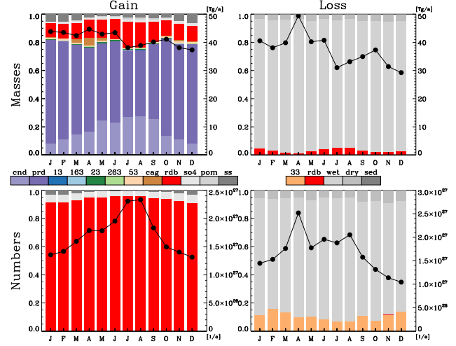
Fig. 18. Seasonal cycle of regional tendencies of the hydrophilic accumulation mode over East-Asia (see Fig. 1). The coloured bars show fractional tendencies (left axis) for the processes defined in Table 2. The solid line (right axis) shows the total tendency.
