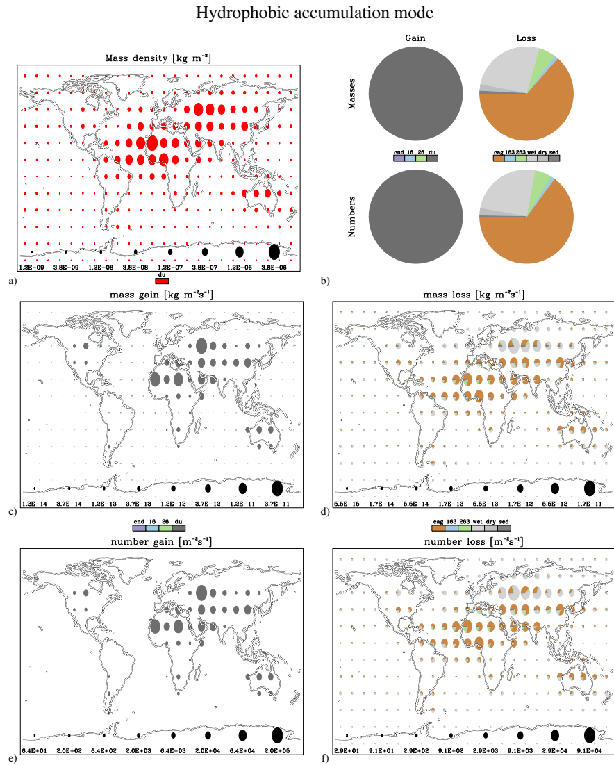
Fig. 14. Global distribution of annual burdens (a) and tendencies (b,c,d,e and f) of the hydrophobic accumulation mode. The colours indicate either species (defined in Table 3) or processes (defined in Table 2). The pie-chart shows fractional contributions, while the radius of the pie indicates total column burden or total column tendency (logarithmic scale as shown in black at the bottom of panels a,c,d,e and f). Panel b shows a global average of the tendencies.
