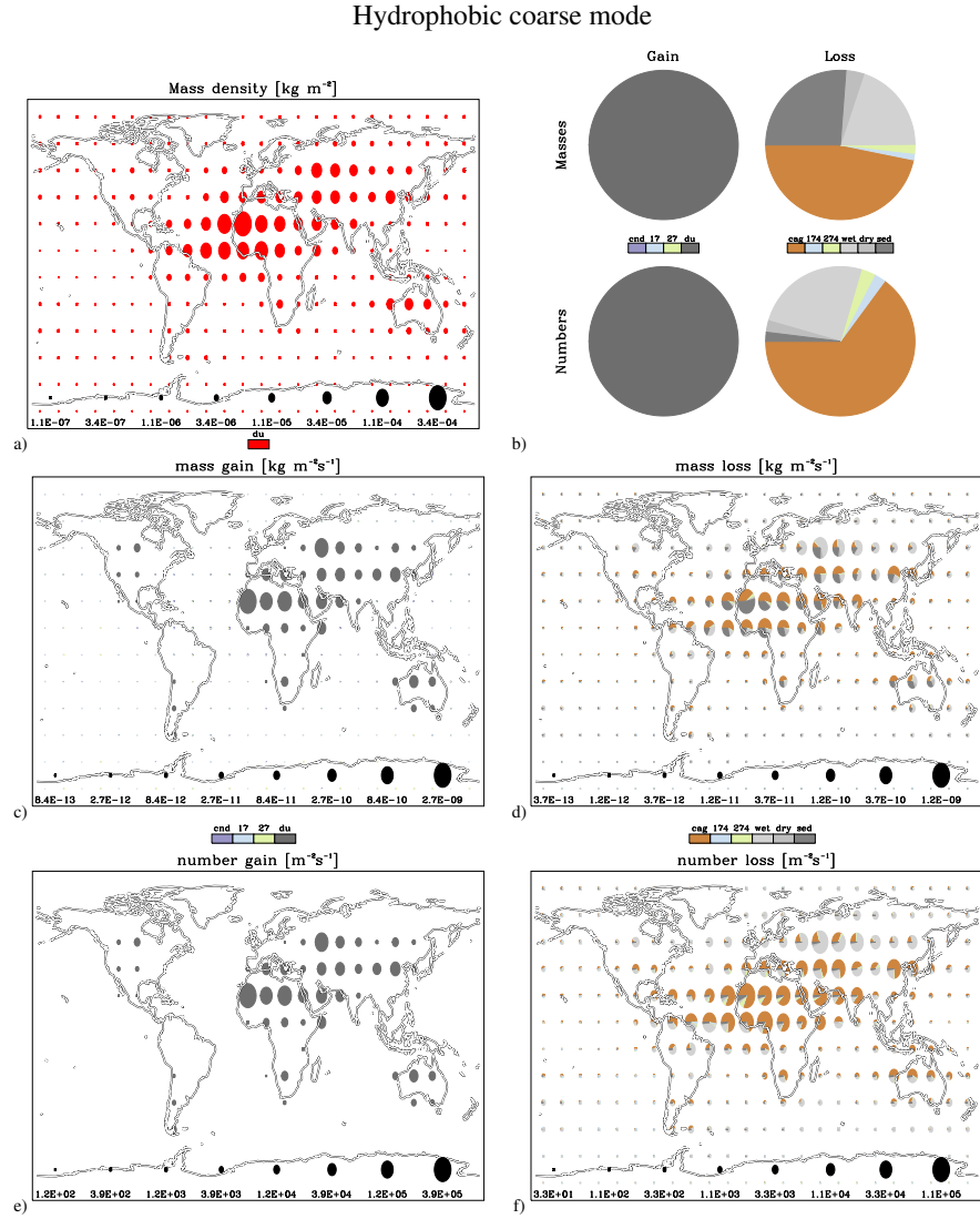
Fig. 20. Global distribution of annual burdens (a) and tendencies (b,c,d,e and f) of the hydrophobic coarse mode. The colours indicate either species (defined in Table 3) or processes (defined in Table 2). The pie-chart shows fractional contributions, while the radius of the pie indicates total column burden or total column tendency (logarithmic scale as shown in black at the bottom of panels a,c,d,e and f). Panel b shows a global average of the tendencies.
