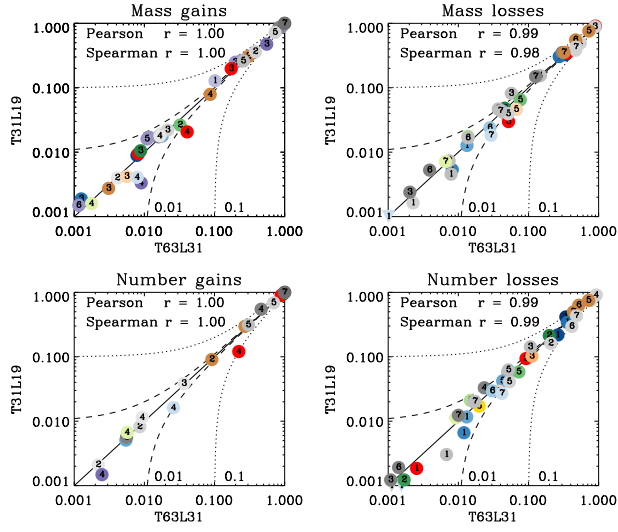
Fig. 24. Fractional tendencies for the T31L19 low-resolution experiment versus the baseline T63L31 high-resolution experiment. Colours indicate processes (Table 2), numbers indicate modes (Table 3). Results are shown for North America.
