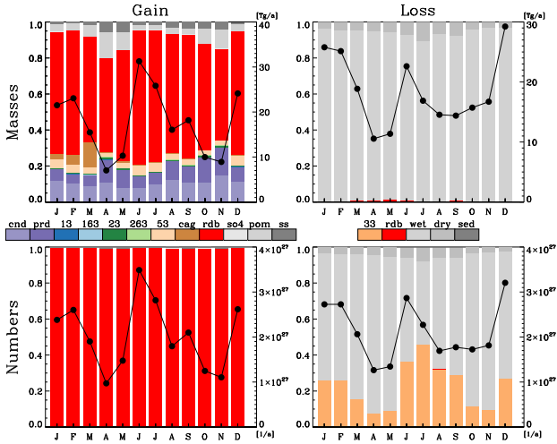
Fig. 17. Seasonal cycle of regional tendencies of the hydrophilic accumulation mode over the Savanna (see Fig. 1). The coloured bars show fractional tendencies (left axis) for the processes defined in Table 2. The solid line (right axis) shows the total tendency.
