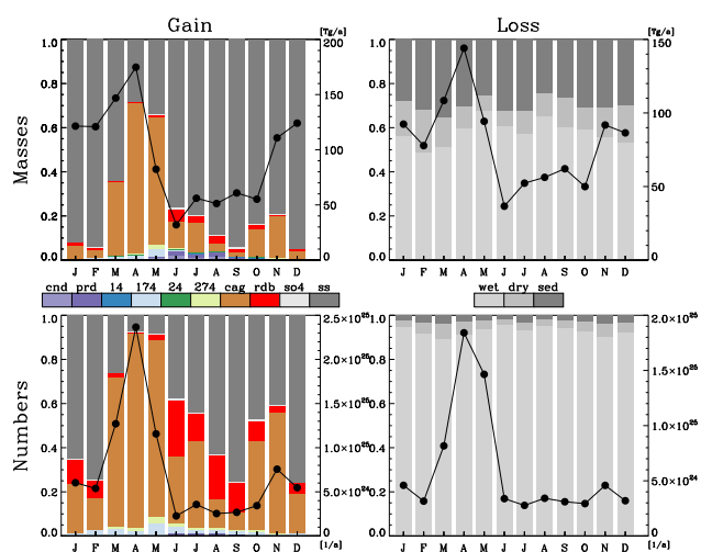
Fig. 23. Seasonal cycle of regional tendencies of the hydrophilic coarse mode over East-Asia (see Fig. 1). The coloured bars show fractional tendencies (left axis) for the processes defined in Table 2. The solid line (right axis) shows the total tendency.
