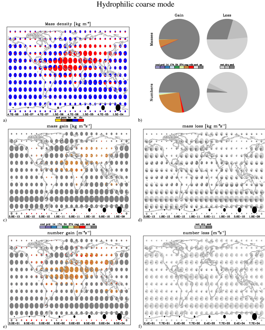
Fig. 22. Global distribution of annual burdens (a) and tendencies (b,c,d,e and f) of the hydrophilic coarse mode. The colours indicate either species (defined in Table 3) or processes (defined in Table 2). The pie-chart shows fractional contributions, while the radius of the pie indicates total column burden or total column tendency (logarithmic scale as shown in black at the bottom of panels a,c,d,e and f). Panel b shows a global average of the tendencies.
