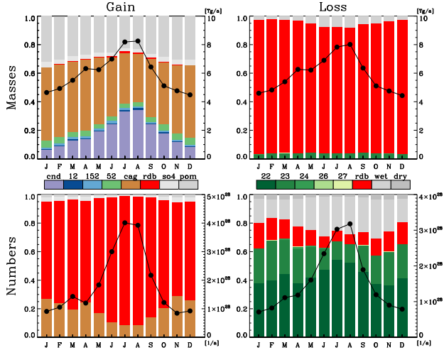
Fig. 13. Seasonal cycle of regional tendencies of the hydrophilic Aitken mode over East-Asia (see Fig. 1). The coloured bars show fractional tendencies (left axis) for the processes defined in Table 2. The solid line (right axis) shows the total tendency.
