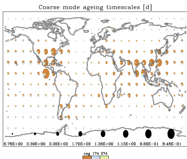
Fig. 21. Ageing time-scales of the hydrophobic coarse mode. This time-scale is defined as N/(\partial N/\partial t) , with N the number density and \partial N/\partial t its time-derivative due to ageing processes only . The colours indicate processes (Table 2), the radius of the pie indicates ageing time-scale (inverse linear scale)
