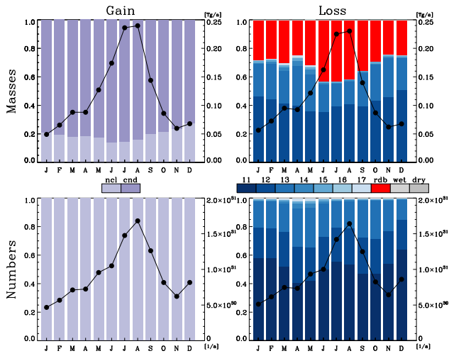
Fig. 7. Seasonal cycle of regional tendencies of the nucleation mode over East-Asia (see Fig. 1). The coloured bars show fractional tendencies (left axis) for the processes defined in Table 2. The solid line (right axis) shows the total tendency.
