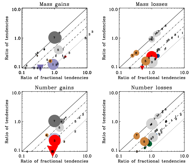
Fig. 26. Pre-industrial (PI) to Present Day (PD) ratios of absolute tendencies against PI to PD ratios of fractional tendencies. Colours indicate processes (Table 2), numbers indicate modes (Table 3). The size of the symbol indicates fractional tendency in the PD experiment, with the largest symbols having a fractional tendency of about 1 (linear scale). The slanted lines represent y = 2^{-n}x , with n = 0, 1, 2, 3 . Results are shown for North America.
