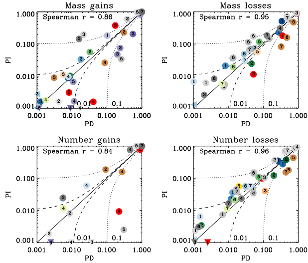
Fig. 25. Fractional tendencies for the Pre-Industrial experiment versus the Present Day experiment. Colours indicate processes (Table 2), numbers indicate modes (Table 3). Results are shown for North America.
