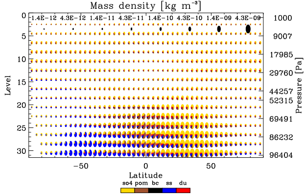
Fig. 16. Zonal distribution of annual densities of the hydrophilic accumulation mode. The colours indicate species (defined in Table 3). The pie-chart shows fractional contributions, while the radius of the pie indicates the zonally-averaged density (logarithmic scale as shown in black at the top).
