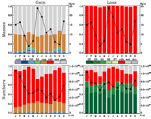
Fig. 12. Seasonal cycle of regional tendencies of the hydrophilic Aitken mode over the Savanna (see Fig. 1). The coloured bars show fractional tendencies (left axis) for the processes defined in Table 2. The solid line (right axis) shows the total tendency.
