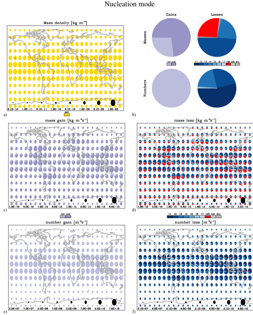
Fig. 5. Global distribution of annual burdens (a) and tendencies (b,c,d,e and f) of the nucleation mode. The colours indicate either species (defined in Table 3) or processes (defined in Table 2). The pie-chart shows fractional contributions, while the radius of the pie indicates total column burden or total column tendency (logarithmic scale as shown in black at the bottom of panels a,c,d,e and f). Panel b shows a global average of the tendencies.
