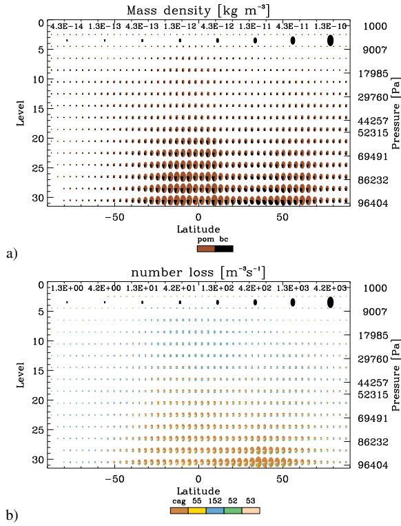
Fig. 9. Zonal distribution of annual densities (a) and tendencies (b) of the hydrophobic Aitken mode. The colours indicate either species (defined in Table 3) or processes (defined in Table 2). The pie-chart shows fractional contributions, while the radius of the pie indicates the zonally-averaged density or tendency (logarithmic scale as shown in black at the top of the panels a and b).
