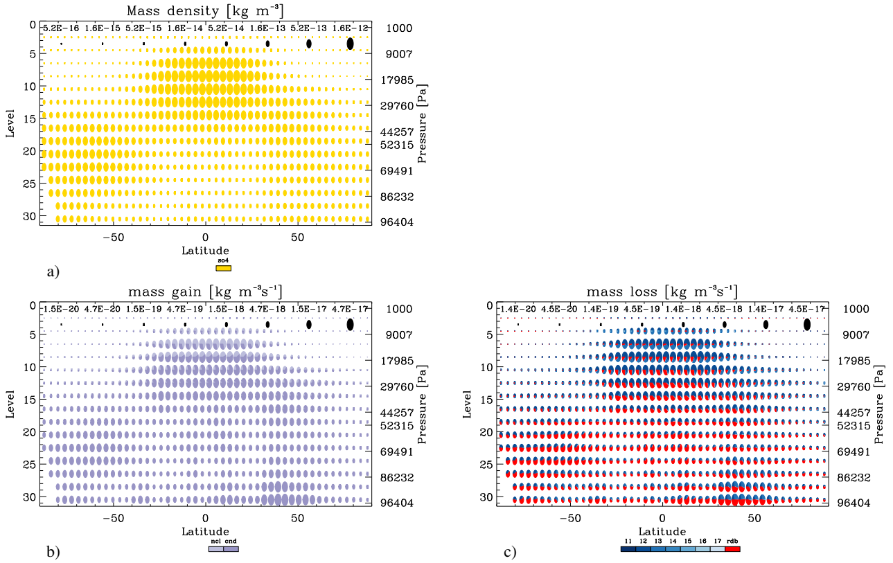
Fig. 6. Zonal distribution of annual densities (a) and tendencies (b and c) of the nucleation mode. The colours indicate either species (defined in Table 3) or processes (defined in Table 2). The pie-chart shows fractional contributions, while the radius of the pie indicates the zonally-averaged density or tendency (logarithmic scale as shown in black at the top of the panels a,b and c).
