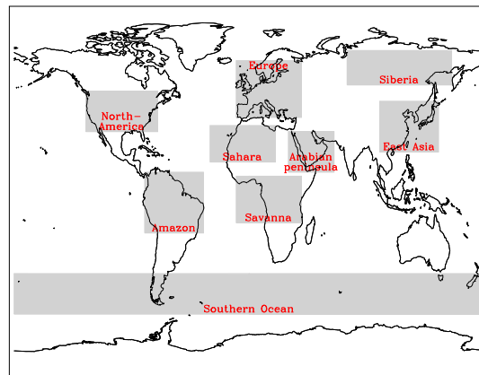
Fig. 1. Definition of the regions that will be used for part of the analysis in this paper.
