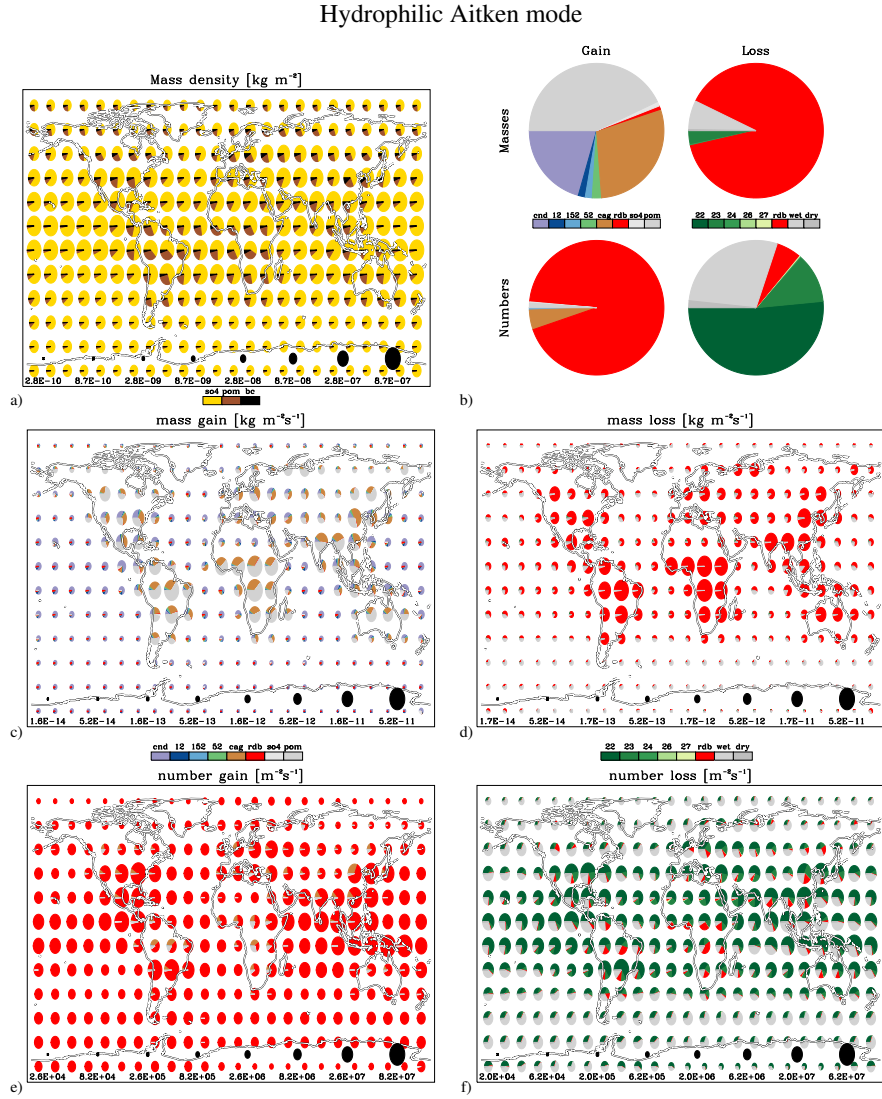
Fig. 11. Global distribution of annual burdens (a) and tendencies (b,c,d,e and f) of the hydrophilic Aitken mode. The colours indicate either species (defined in Table 3) or processes (defined in Table 2). The pie-chart shows fractional contributions, while the radius of the pie indicates total column burden or total column tendency (logarithmic scale as shown in black at the bottom of panels a,c,d,e and f). Panel b shows a global average of the tendencies.
