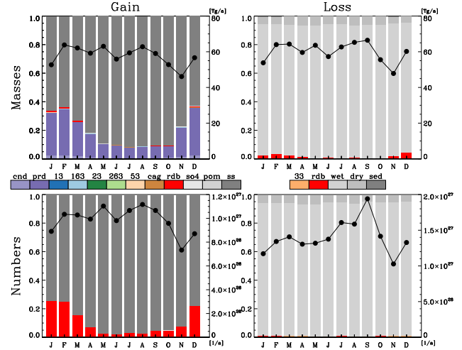
Fig. 19. Seasonal cycle of regional tendencies of the hydrophilic accumulation mode over the southern ocean (see Fig. 1). The coloured bars show fractional tendencies (left axis) for the processes defined in Table 2. The solid line (right axis) shows the total tendency.
