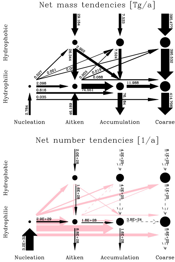
Fig. 4. Globally and annually averaged net mass and number tendencies (arrows) between the 7 modes (dots) in ECHAM5.5-HAM2. The vertical arrows at the top and bottom of the figure represent \text{H}_2\text{SO}_4 nucleation, condensation & production, aerosol primary emission and deposition processes. The arrows between the modes represent coagulation, ageing and redistribution processes. Pink arrows are number loss tendencies for coagulation processes. The width of the arrow scales logarithmically with the magnitude of the net tendency. In addition, numerical values for the annual and global averages are given.
