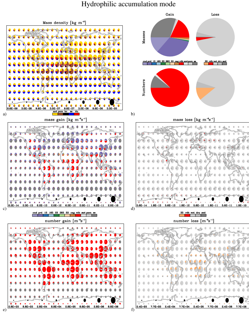
Fig. 15. Global distribution of annual burdens (a) and tendencies (b,c,d,e and f) of the hydrophilic accumulation mode. The colours indicate either species (defined in Table 3) or processes (defined in Table 2). The pie-chart shows fractional contributions, while the radius of the pie indicates total column burden or total column tendency (logarithmic scale as shown in black at the bottom of panels a,c,d,e and f). Panel b shows a global average of the tendencies.
