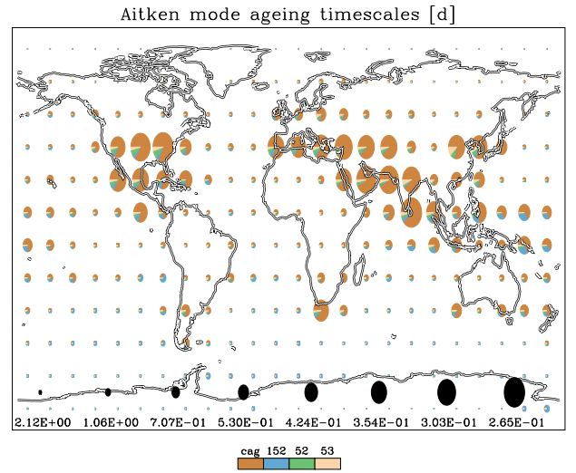
Fig. 10. Ageing time-scales of the hydrophobic Aitken mode. This time-scale is defined as N/(\partial N/\partial t) , with N the number density and \partial N/\partial t its time-derivative due to ageing processes only . The colours indicate processes (Table 2), the radius of the pie indicates ageing time-scale (inverse linear scale)
