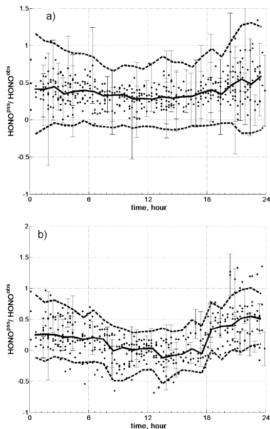
Figure 9. Ratio of PSS calculated and measured [HONO]: (a) from OH budget; (b) from net radical (OH and RO 2 ) sources and sinks. Solid lines – median values; dashed lines- upper and lower quartiles of the mean values with added standard deviations, respectively. Error bars correspond to standard deviation.
