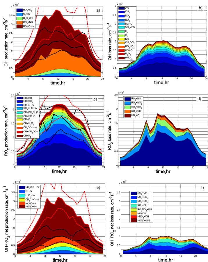
Figure 5. Median diurnal production and loss rates of OH (a, b), RO 2 (c, d) and net production and loss rates of radicals OH+RO 2 (e, f). Solid red and black lines represent the total production and loss rates, respectively. Dashed lines correspond to corresponding quartiles.
