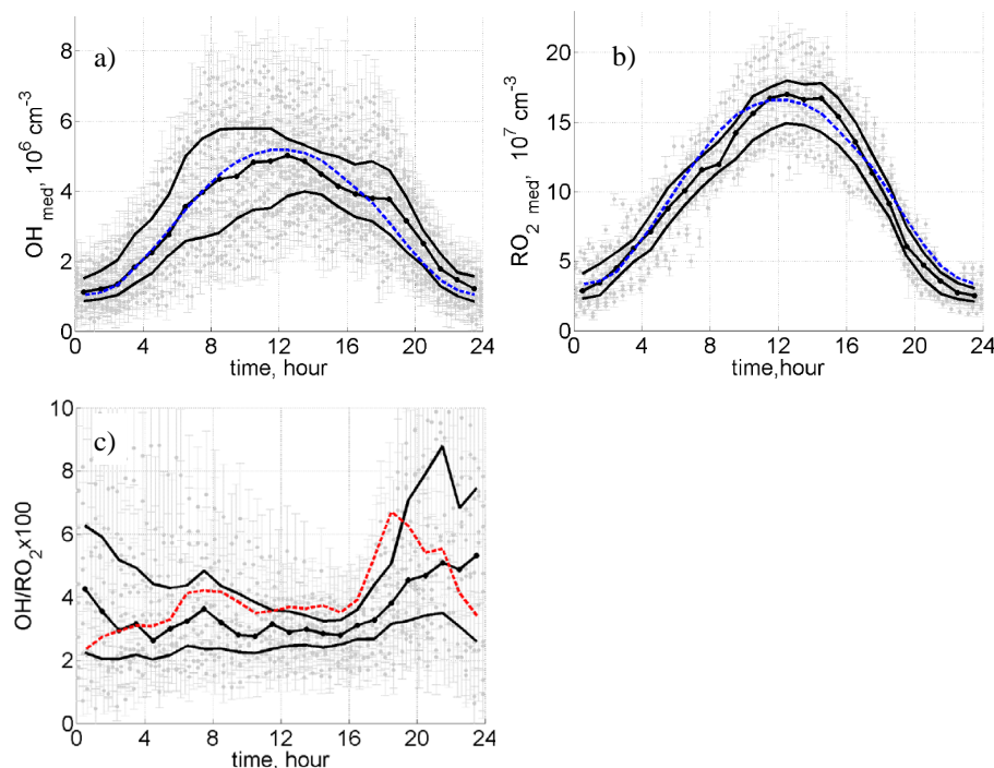
Figure 2. Median diurnal concentration profiles of OH (a), RO 2 (b) and [OH]/[RO 2 ] ratio (c). Solid lines represent the median and quartile levels. Points – 15 min averaged measured values with standard deviations. Blue lines in (a) and (b) represent J(\text{NO}_2) in arbitrary units. Red line in (c) represents median NO in arbitrary units.
