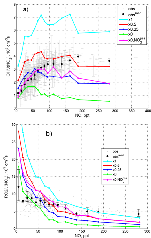
Figure 4. Normalized concentrations of OH (a) and RO 2 (b) vs. measured concentrations of NO. Grey and black points represent observations; colored lines – MCM calculations with [HONO] multiplied by a factor presented in Figure legends. Magenta – [HONO] = 0 and [NO 2 ] is calculated by assuming PSS ratio of [NO 2 ]/[NO].
