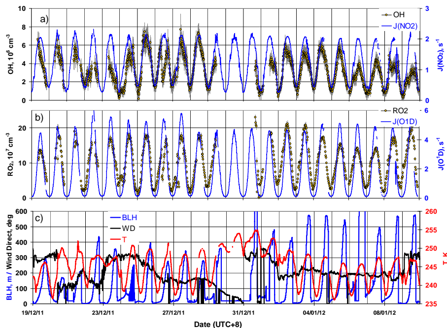
Figure 1. Time series of [\text{OH}] and J(\text{NO}_2) (a), [\text{RO}_2] and J(\text{O}^1\text{D}) (b), Wind Direction (WD), Temperature ( T ) and modelled Boundary Layer Height (BLH) (c) data for the campaign at Dome C.
