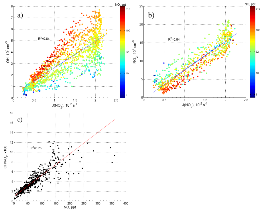
Figure 3. Correlations of [OH] (a) and [RO 2 ] (b) with J(\text{NO}_2) and of the ratio of [OH]/[RO 2 ] with [NO] (c).
