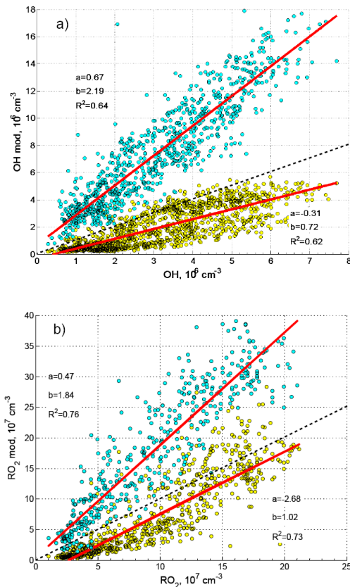
Figure 7. Correlation of 0-D modelled vs. measured [OH] (a) and [RO 2 ] (b) . The model is constrained by [HONO] = 0 (yellow) or by measured [HONO] (blue). Coefficients a , b correspond to intercepts and slopes, respectively. Black lines correspond to linear dependences with a = 0 and b = 1 .
