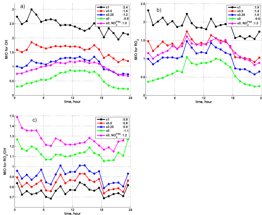
Figure 8. Median diurnal Model(0-D)/Observation ratios (M/O) for [OH], [RO 2 ] and [RO 2 ]/[OH] for the model constrained by [HONO] taken as measured or reduced by factors 0.5, 0.25, and equal to zero. The “HONO = 0, NO 2 PSS ” curves correspond to the model with [HONO] = 0 and [NO 2 ] calculated assuming [NO x ] at PSS. Numbers in legends represent diurnal median M/O ratios.
