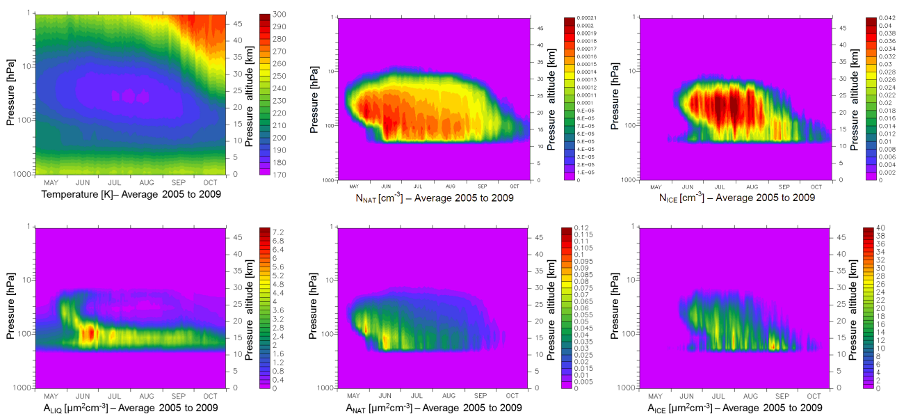
Fig. 2. Stratospheric temperature, liquid and solid particles – time series averaged from 80° to 90° S and over the years 2005 to 2009 for temperature in K (top left), number densities of NAT ( N_{NAT} ) and ice particles ( N_{ICE} ) in \text{cm}^{-3} (top center and right), as well as surface area densities of liquid particles ( A_{LIQ} ), NAT ( A_{NAT} ) and ice particles ( A_{ICE} ) in \mu\text{m}^2\text{cm}^{-3} (bottom left to right). The results shown are valid for the standard and for all three sensitivity simulations.
