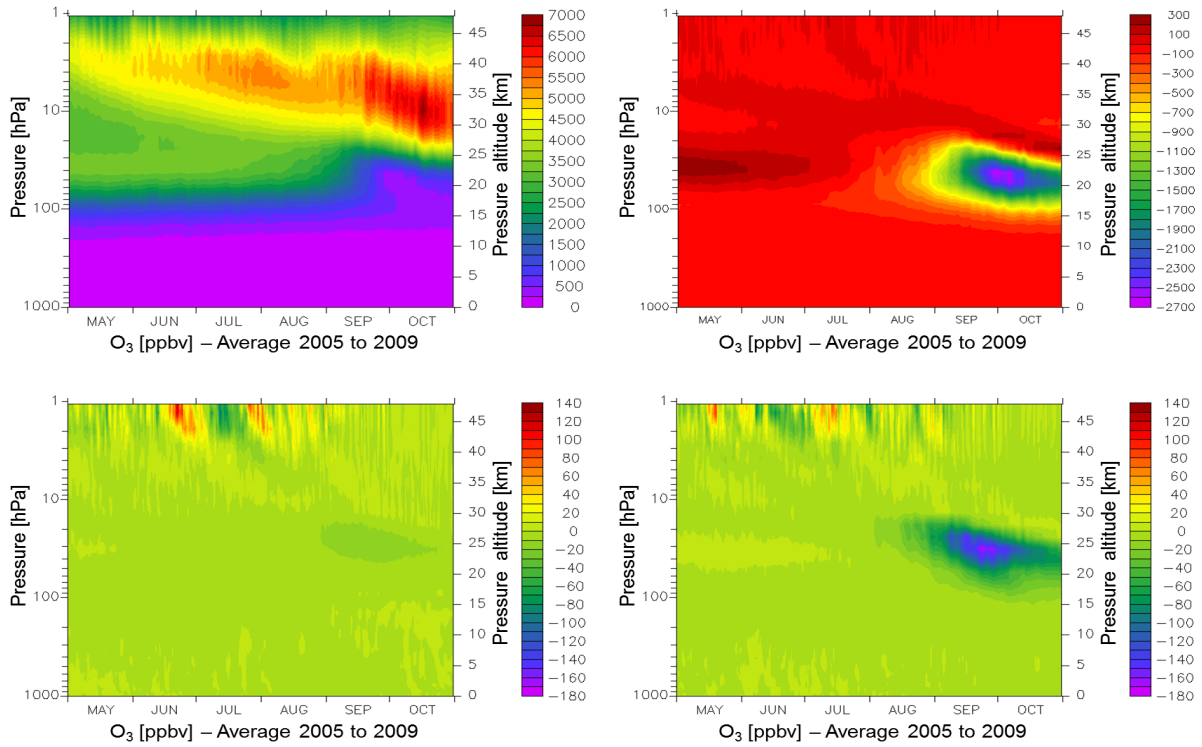
Fig. 5. Ozone depletion – time series of O 3 in ppbv in the standard EMAC simulation during Antarctic winter and spring averaged over 80° to 90° S and the years 2005 to 2009 (top left) and contribution of liquid particles (top right), additional NAT particles (bottom left) and additional ice particles (bottom right). Note that the color bars have different units.
