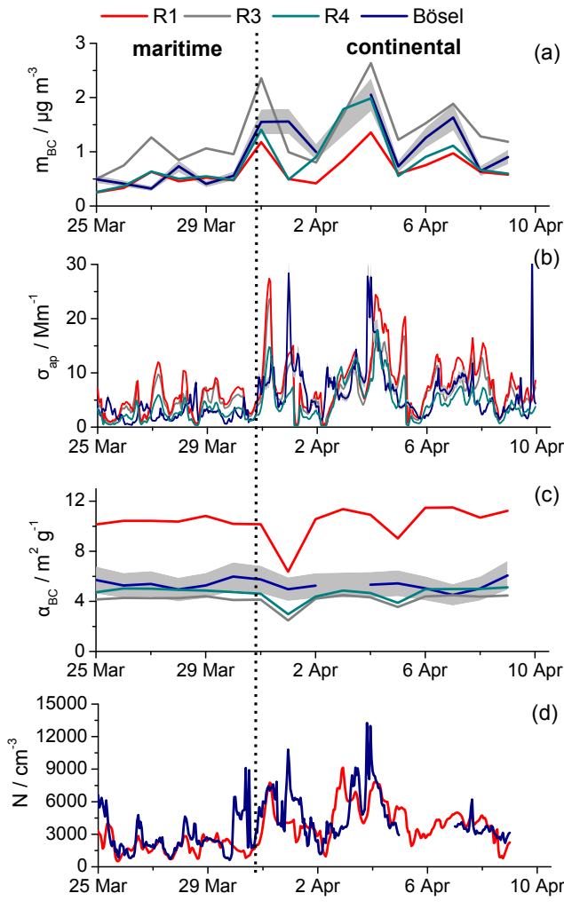
Fig. 3. Comparison between measured C_{\text{soot}} and modelled BC mass concentrations ( m_{BC} ) (a), absorption coefficient ( \sigma_{ap} ) (b), mass absorption cross-sections ( \alpha_{BC} ) (c) and particle number concentration ( N ) (d) at the regional observation site Bösel. Besides the results for model base run R1, the time series from additional model runs R3 and R4 are also shown, which differ from R1 in the EC emissions and the calculation of optical properties (see Table 2).
