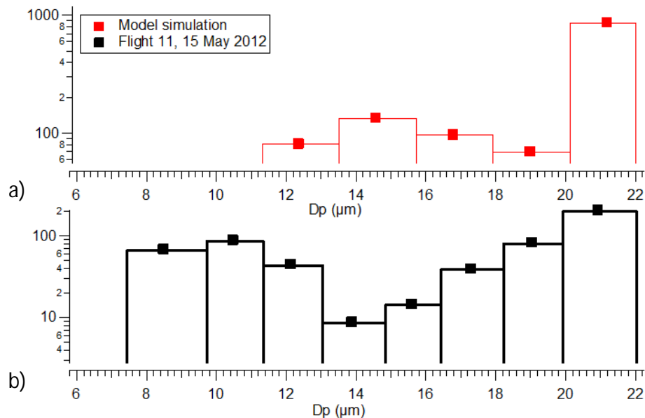
Figure 13. (a) A bimodal SD of the modeled droplets from the last 70 m of the simulated plane trajectory in comparison with (b) bimodal SD of the measured droplets during Flight 11 (see Fig. 5c).
