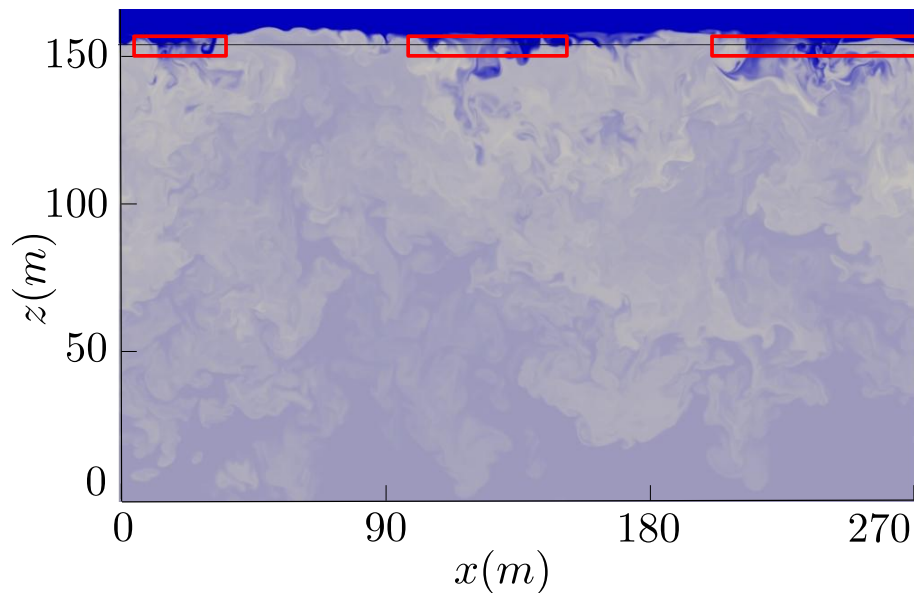
Figure 11. Vertical cross section of the simulated cloud liquid water. The black line indicates the trajectory of the simulated plane and the red rectangles mark the cloud holes. The color scale goes from 0.0 \text{ g kg}^{-1} (blue) to 0.325 \text{ g kg}^{-1} (white).
