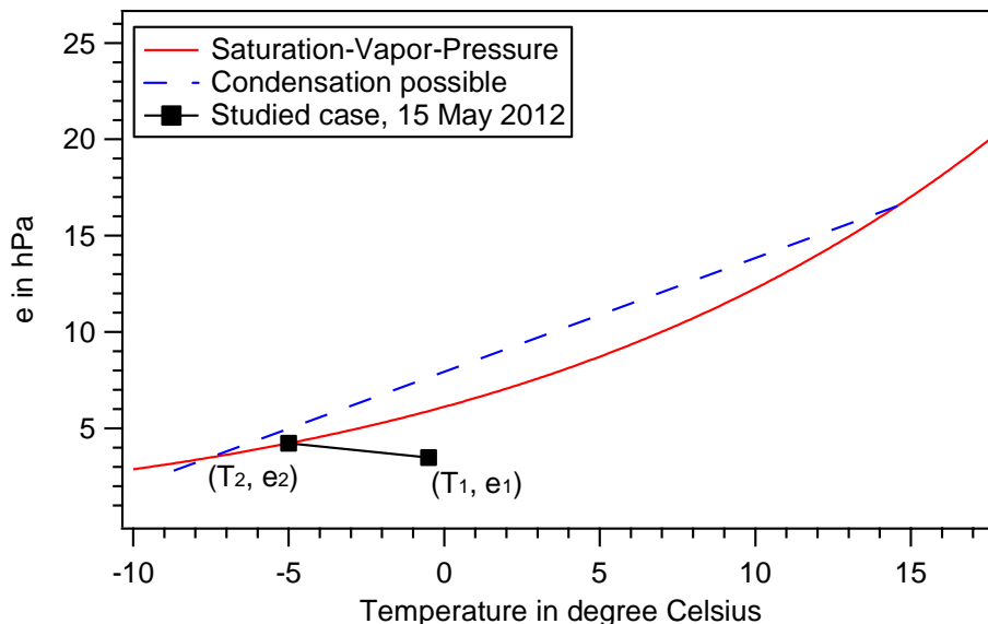
Figure 10. Isobaric mixing between a cloud and a dry air parcel. The studied case from 15 May 2012 is represented by the straight line. The thermodynamic parameters T_1 = -0.5^\circ\text{C} , \text{RH}_1 = 59\% , e_1 = 3.5 hPa for dry air and T_2 = -5^\circ\text{C} , \text{RH}_2 = 100\% , e_2 = 4.2 hPa inside the cloud are based on the measurements. Isobaric condensation occurs when in mixing of two parcels results in a composition that lays below the condensation line, due to the nonlinearity (or curvature) in the saturation-vapor-pressure function. The dashed line in the figure illustrates such a mixing process. However, the temperature range covered by our measurements (shown by the continuous line) is so small that the saturation-vapor-pressure is almost linear in this range. As a consequence, condensational mixing is very unlikely and cannot play an important role for generating the second mode in the bimodal SDs.
