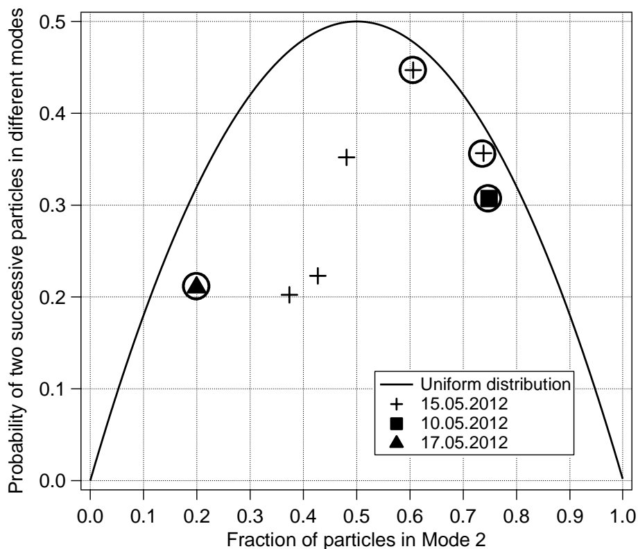
Figure 9. Evaluation of the bimodal SDs. The black line shows a uniform distribution between both size modes. The results from Fig. 8 (60.6 %, 44.7 %) indicate that the bimodal SD is close to an uniform distribution. All in all, four bimodal SDs show a good agreement with the uniform distribution (marked by circles). The agreement for the other bimodal SDs is weak.
