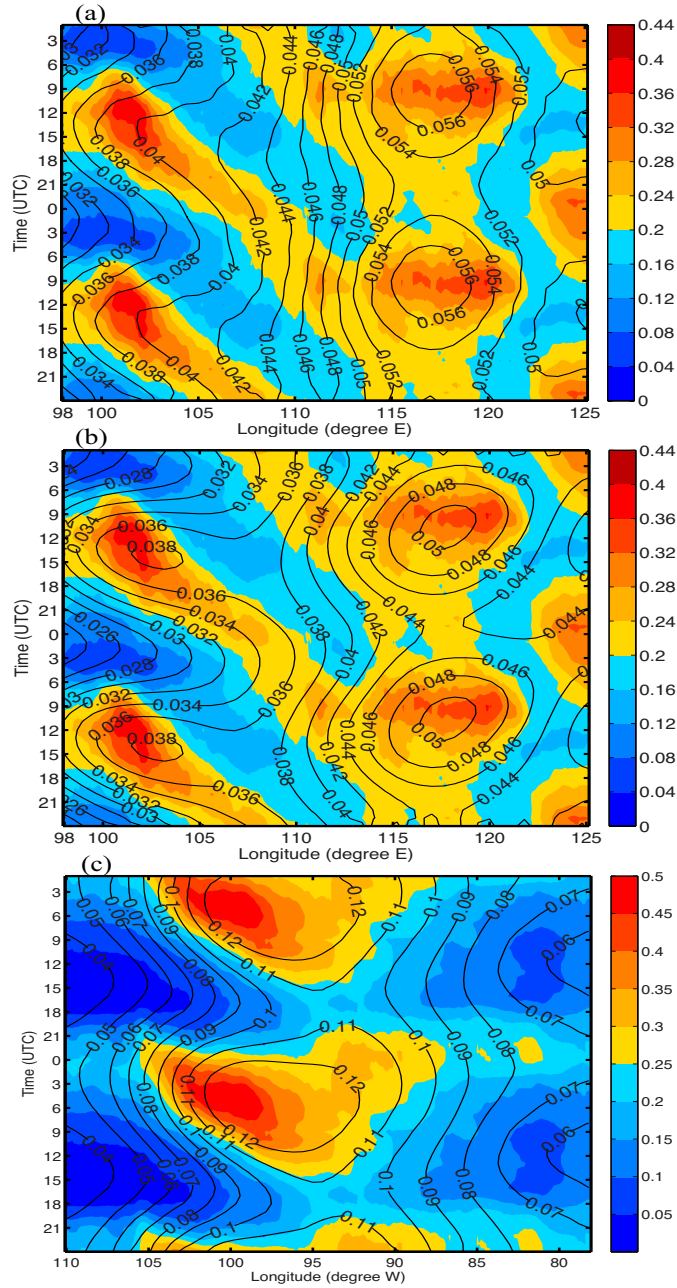
Figure 18. Time-longitude diagram of the diurnal variation in the hourly precipitation (shadings) and the filtered precipitation perturbation variances (contours) for (a) SR3 and (b) SR4 over East Asia, contours interval is 0.02 and (c) for with SR3 for North America, contours interval is 0.01.
