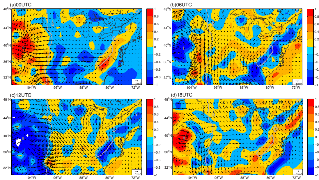
Supplementary Figure: Spatial distribution of the 850-hPa vertical motion derivations ( \text{cm s}^{-1} , colors) and perturbation wind vectors diagnosed with the GFS analyses at (a) 00, (b) 06, (c) 12, and (d) 18 UTC averaged over the warm-season over the domain of 30-48°N, 110-70°W.
