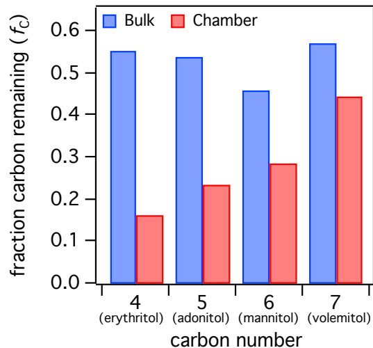
Figure 5. The fraction of carbon remaining in the condensed phase after oxidation ( f_C ) in the bulk solution (blue bars) or in submicron particles (red bars), as calculated from Eq. (2). Meaningful values could not be determined for the oxidation of glycerol (C3) due to evaporation from the particle phase prior to oxidation.
