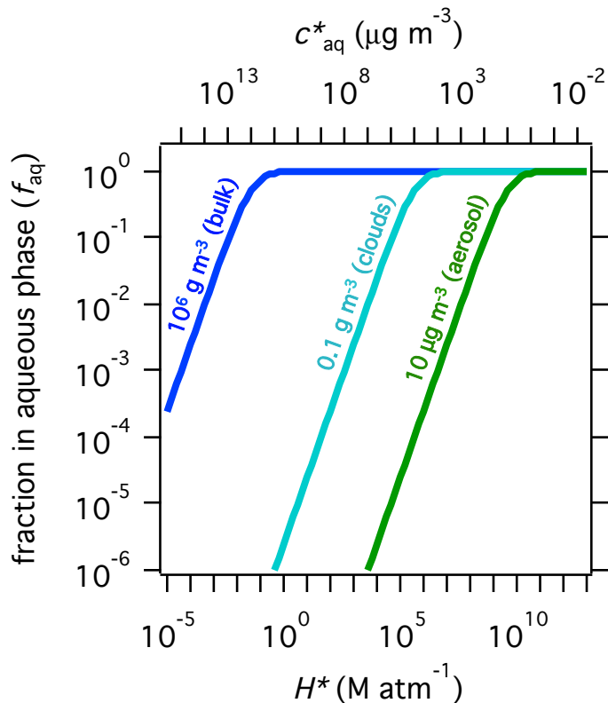
Figure 1. The fraction of a compound that will partition to the aqueous phase ( f_{aq} ) as a function of its Henry's Law constant, H^* (or alternatively its saturation vapor concentration, c_{aq}^* ), and the liquid water content (LWC). Compounds with 1 \text{ M atm}^{-1} < H^* < 10^9 \text{ M atm}^{-1} will be primarily in the aqueous phase at bulk LWC (blue line), but primarily in the gas phase at aqueous aerosol LWC (green line). Cloud water (teal line) represents the intermediate case, with more partitioning into the aqueous phase than for aqueous particles, but still with far less than for a bulk aqueous solution.
