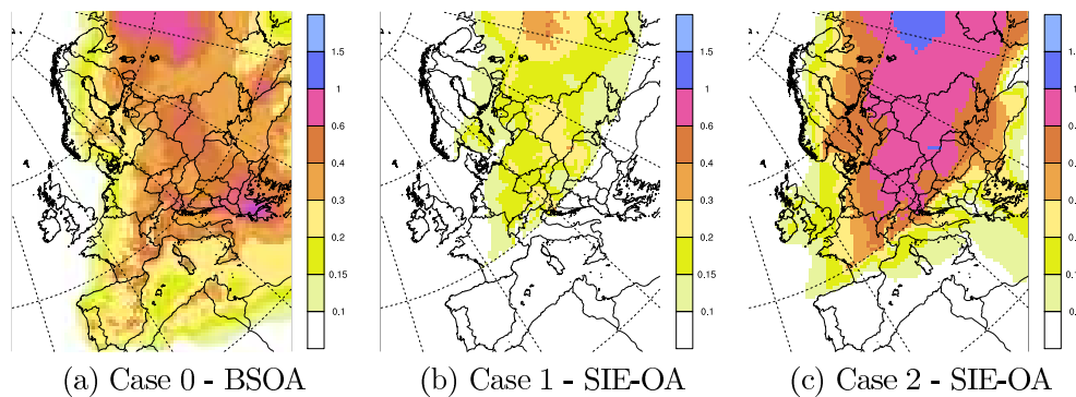
Fig. 4: Model calculated 6-month mean (Apr-Sep) concentrations of BSOA and biotic stress induced OA (SIE-OA); (a) BSOA in Case 0 (reference case with minor stress induced emissions), (b) SIE-OA in Case 1 (biotic stress with sesquiterpene (SQT) emissions), (c) SIE-OA in Case 2 (biotic stress with emissions of SQT and methyl salicylate). Unit: \mu g m^{-3} .
