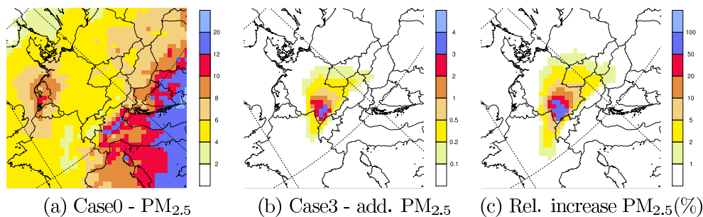
Fig. 8: Model calculated regional background PM_{2.5} concentration (2-month-mean for June-July). (a) Total model PM_{2.5} with minor biotic stress (Case 0) [ \mu\text{g m}^{-3} ]; (b) Additional PM_{2.5} due to organic aerosol formation caused by biotic stress induced emissions in Case 3 (infestation of Spruce in Baden-Württemberg by Cinara Pilicornis ) [ \mu\text{g m}^{-3} ]; (c) Relative increase in modelled regional background PM_{2.5} [in %] due to the simulated infestation.
