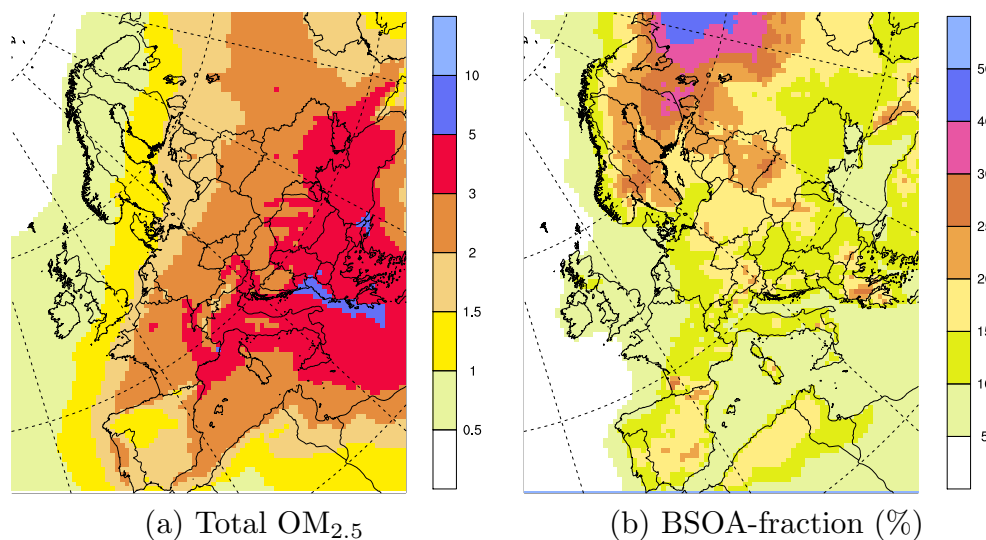
Fig. 3: Model calculated 6-month mean (Apr-Sep) concentrations of (a) total Organic Matter in PM_{2.5} ( OM_{2.5} ) [Unit: \mu g m^{-3} ] and (b) Fraction of biogenic secondary organic aerosol (BSOA) [% of total OM_{2.5} ] for the reference scenario assuming only minor biotic stress (Case 0).
