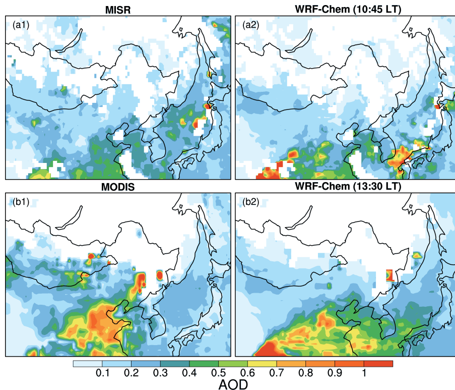
Figure 8. Spatial distribution of AOD over North China in January–February of 2010 from the MISR and Aqua-MODIS retrievals and the corresponding WRF-Chem simulations. The model results are sampled at the MISR (~ 10:45 LT) and Aqua-MODIS (~ 13:30 LT) overpass time, respectively, at the locations where retrievals are available.
