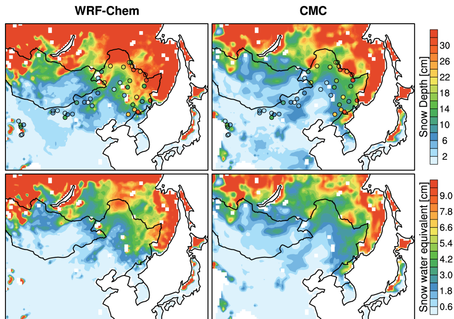
Figure 2. Spatial distribution of snow depth (cm) and snow water equivalent (cm) from the WRF-Chem simulations and CMC reanalysis over North China in January–February of 2010. Snow depth (cm) from the campaign observations (colored circle) is also shown.
