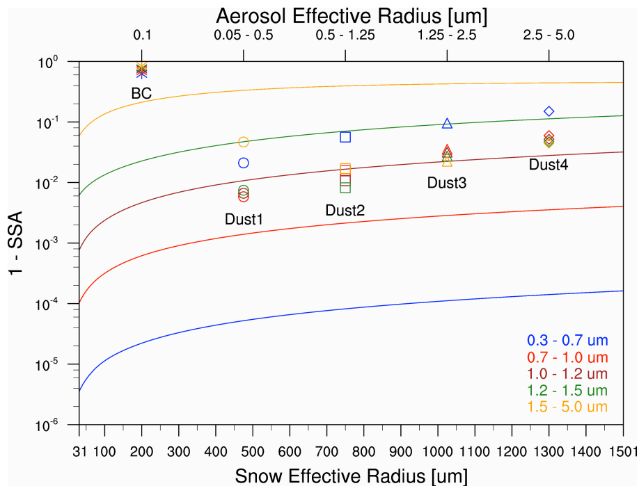
Figure 11. Single scattering albedo (SSA) complement ( 1-SSA ) at the five spectral wavebands of snow grains as a function of effective radius (colored solid lines), BC with an effective radius of 0.1 \mu\text{m} (asterisk), and dust with four different sizes (Dust1 (circle), Dust2 (square), Dust3 (triangle), and Dust4 (diamond)).
