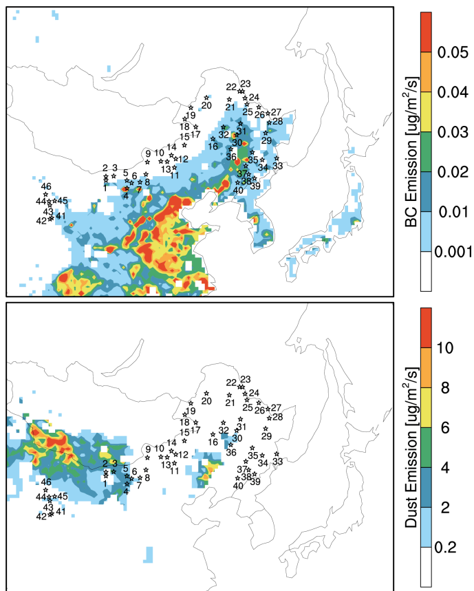
Figure 1. Model domain with BC and dust emissions in January–February of 2010. The 46 observation sites in the North China campaign are denoted by pentagrams in black.
