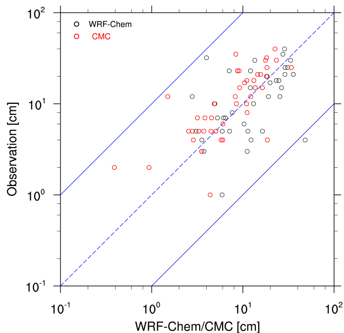
Figure 3. The campaign observations of snow depth (cm) vs. the corresponding WRF-Chem simulations (black dots) and CMC reanalysis (red dots).
