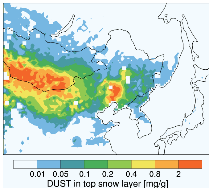
Figure 9. Spatial distribution of dust mass concentration in the top snow layer from the WRF-Chem simulations over North China in January–February of 2010.
