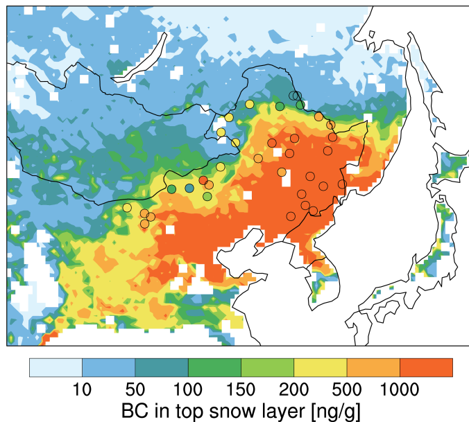
Figure 5. Spatial distribution of BC mass concentration in the top snow layer from the WRF-Chem simulations over North China in January–February of 2010. The campaign observed BC mass concentrations in the top snow layer (colored circle) are also shown.
