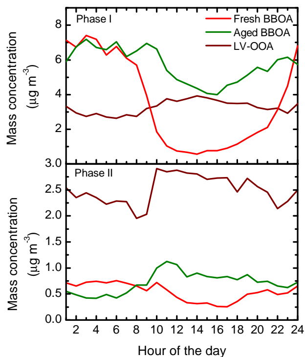
Fig. 12. Diurnal variation of the three factors identified through PMF: Fresh BBOA, Aged BBOA and LV-OOA. Phase I refers to the period between 13 to 22 September and Phase II from 22 to 30 September 2012.
