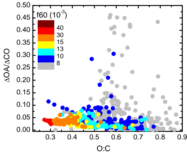
Fig. 8. \Delta OA/\Delta CO mass ratios versus O:C ratio.
