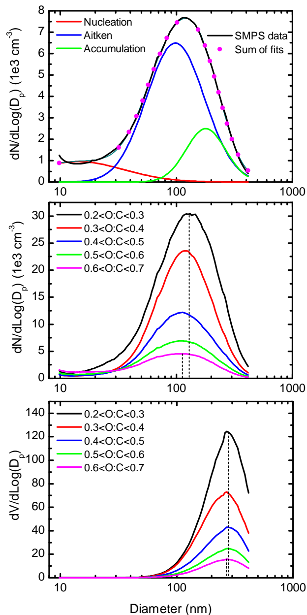
Fig. 9. Top: Average aerosol size distribution observed at ground level during SAMBBA. The average particle number concentration and diameter were 5\,800\text{ cm}^{-3} and 94.4 nm, respectively. Log-normal fit parameters are shown in Table 2. Middle: solid line shows the average number size distribution based on different O : C ranges. The dashed line indicates size distribution centroid for fresh (130 nm) and aged aerosol (110 nm). Bottom: solid line shows the average volume size distribution based on different O : C ranges. The dashed line indicates size distribution centroid for fresh (278 nm) and aged aerosol (267 nm).
