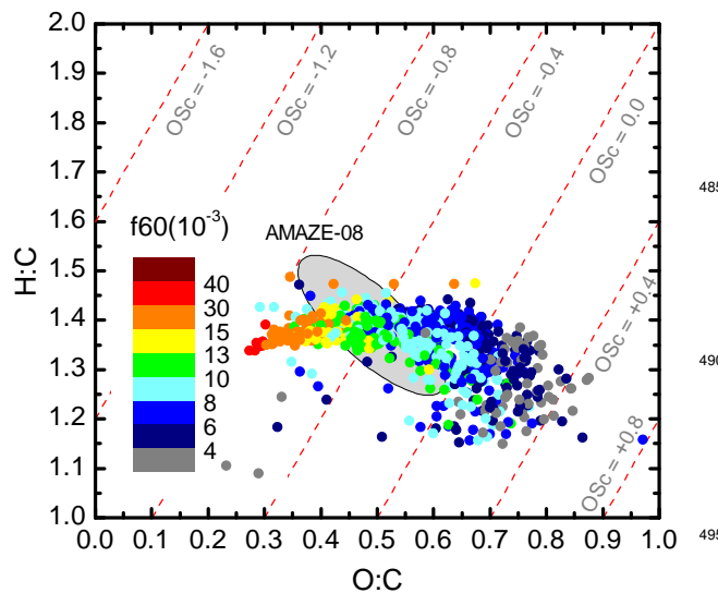
Fig. 7. Representation of the OA components into the VK-triangle diagram. The estimated carbon oxidation states ( \overline{OS}_C \approx 2 \times O/C - H/C ) are shown as red dotted lines. Gray area indicates the V-K space from AMAZE-08 as described by Heald et al. (2010).
