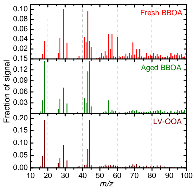
Fig. 10. Mass spectra in fraction of signal of PMF factors, Fresh BBOA, Aged BBOA and LV-OOA.
