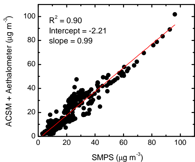
Fig. 2. Comparison between the sum of the mass concentrations of species measured by the ACSM and Aethalometer (at 880 nm) versus integrated mass concentration obtained from SMPS.
