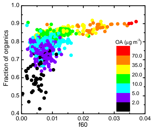
Fig. 6. The fraction of organic aerosol relative to total mass (non-refractory and BC_e ) versus f_{60} , a marker for biomass burning impacted air masses.
