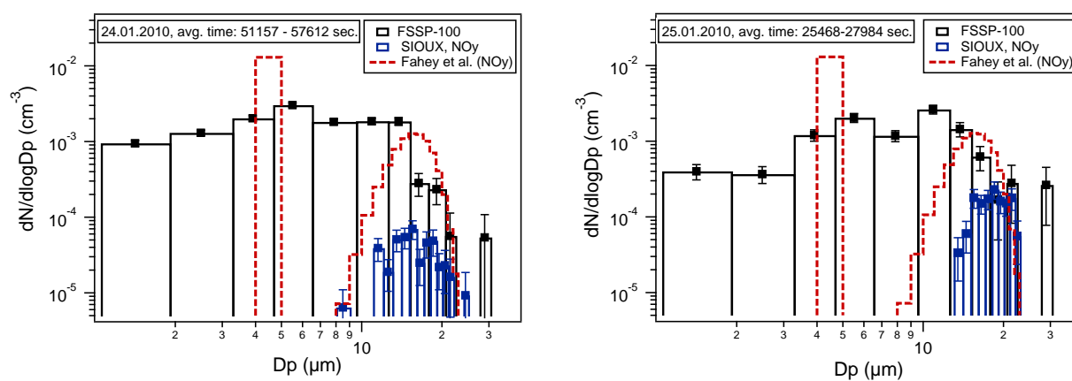
Fig. 013. Size distributions of the FSSP-100 data for time intervals where the total \text{NO}_y data of the SIOUX instruments allowed extraction of particle data from single peaks, and for which diameters assuming NAT composition were derived. The sensitivity of the \text{NO}_y instrument scales with particle volume, so that sizes only above about 10\mu\text{m} could be retrieved. A particle size independent enhancement factor was used, which might explain some of the discrepancy in the particle numbers between the \text{NO}_y and the optical measurements.
