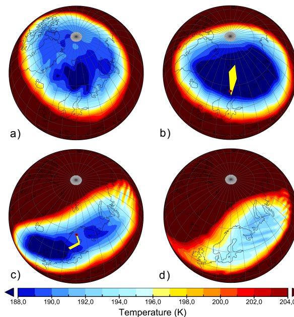
Fig. 01. ERA Interim data of temperature at 30 hPa level during RECONCILE in January 2010: (a) 10 January 00:00 UTC (b) 17 January 12:00 UTC – corresponds to 1st PSC flight. Here the measurement region of the first four flights (17–24 Jan) is marked as yellow area. (c) 25 January 12:00 UTC – last flight with PSC occurrence as indicated with the flight track. (d) 28 January 18:00 UTC. The darkest blue color in the plot is scaled for temperature below 188 K to illustrate regions with temperatures close to, or below T_{ICE} .
