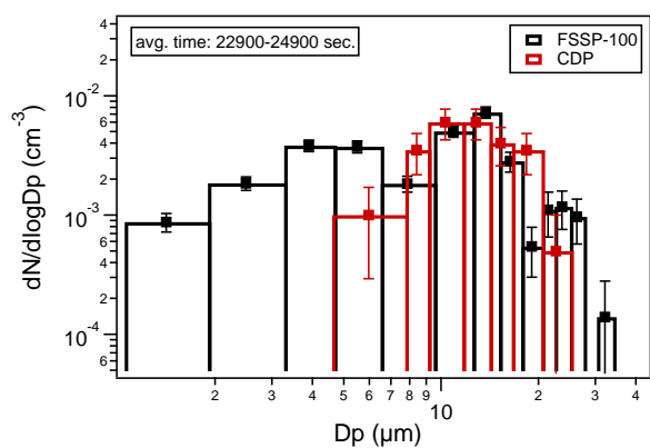
Fig. 07. Size distributions of the FSSP-100 and CDP measured on the flight on 25 January 2010. Due to instrumental problems only in this one flight of the RECONCILE-campaign the particles detection of the CDP worked well with a higher than usual detection size limit of about 5-8 \mu\text{m} . At the same time the largest PSC-particles in relatively high numbers were present in this flight. Note though that the FSSP-size bins above 30 \mu\text{m} contain only 3 counts.
