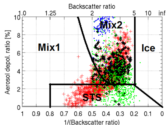
Fig. 010. Scatterplot of aerosol depolarization ratio versus backscatter ratio as measured by the lidars MAL1 and MAL2 (red crosses) on 20 January (see Figure 05), and near in situ by the backscatter-sonde MAS, on 17 January 2010 (green squares), 20 January (black crosses), 25 January (blue squares). The black lines are phase boundaries for different (lidar) PSC types adopted from the scheme described in Pitts et al. (2011). Mix 1 and Mix 2 are mixtures of liquid droplets and solid NAT particles defined for different number densities of NAT particles. Mix 2 represents NAT number densities above 10^{-3} \text{ cm}^{-3} .
