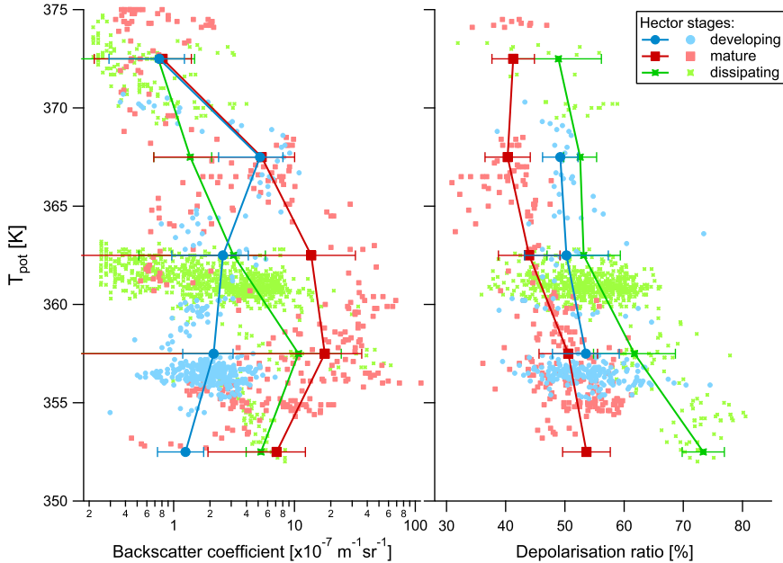
Figure 9. MAS cloud particle backscatter coefficient (left) and cloud particle depolarisation ratio (right). The light coloured markers indicate the individual measurements. Lines and markers represent the averages for the 5 K altitude bins as in Fig. 7 with error bars denoting the standard deviation.
