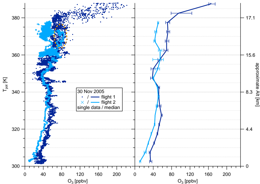
Figure 6. Profiles of ozone mixing ratios from first and second flight on 30 November 2005. Individual (1 Hz) data points are shown in the left panel, median and 33/67 percentiles in the right panel. The orange ellipse encloses data points that were recorded at the beginning of the second flight at the eastern edge of the flight path. The number of these points is much lower than those at later times of the flight, thus, these observations have no visible effect on the median as shown in the right panel.
