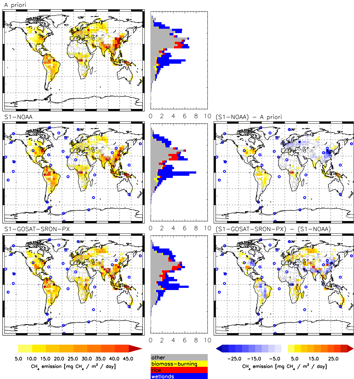
Fig. 6. Left: a posteriori two-year average emissions for S1-NOAA and S1-GOSAT-SRON-PX. The a priori emissions are shown in the topmost plot. White areas indicate grid cells with very low emissions (less than 5 mg CH 4 m -2 day -1 ). Rightmost panels: for S1-NOAA the difference between posteriori and a priori emissions is shown, while for all satellite inversions the panels show the difference between the a posteriori emissions of these inversions and S1-NOAA. The middle plots show the partitioning among the four source categories that have been optimized in this study (two-year latitudinal averages).
