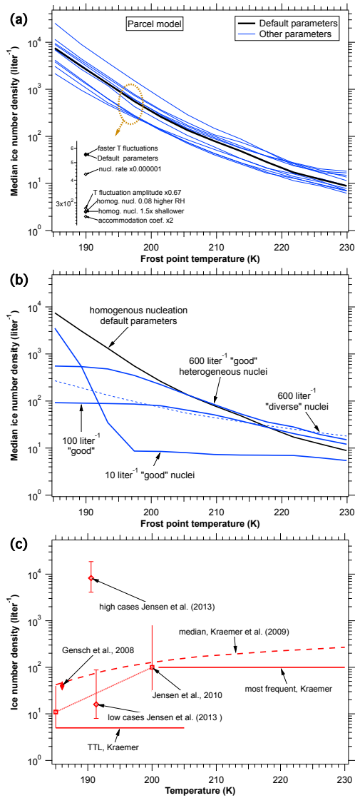
3 Figure 2. Parcel model results for the temperature dependence of ice crystal number 4 density along with results from observations. In (b), “good” heterogeneous nuclei freeze 5 at an ice supersaturation of 1.3 \pm 0.02 whereas “diverse” nuclei are uniformly distributed 6 between supersaturations of 1.3 and 1.65. (c) shows observations described in Gensch et 7 al., 2008, Krämer et al., 2009, Jensen et al., 2010, Jensen et al., 2013b, and typical values 8 from Krämer, personal communication, 2014. Ranges in (c) are approximated from the 9 data in the Jensen et al. papers. In this temperature range homogeneous freezing occurs 10 about 3 K below the frost point.
