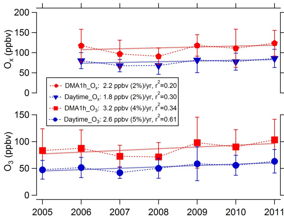
Figure 1 (Upper) Variations in daytime averages (blue triangles) and daily maximum averages (red pentagons) of total oxidants ( O_x ); (Lower) Variations in daytime averages (blue dots) and daily
