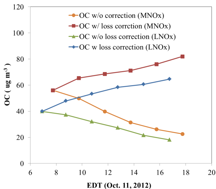
Figure R1. Comparison of OC mass concentrations with wall-loss correction and without correction
