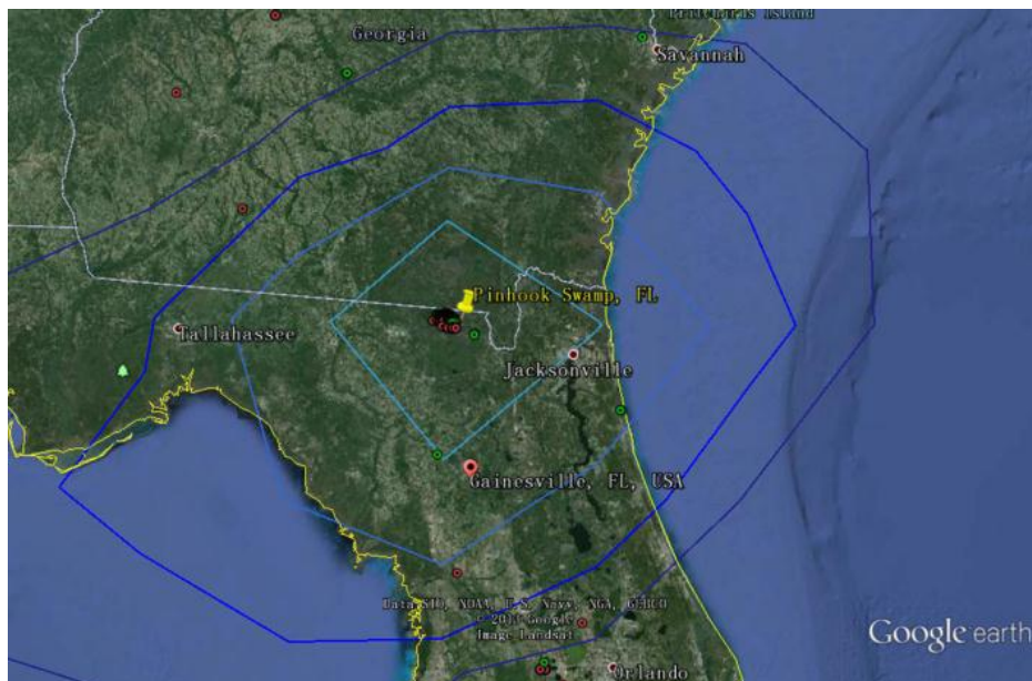
Figure R3. Flambe/MODIS/Cloud/NAAPS data for 09, April, 2012 (County Line Wildfire). The lighter in blue color, the higher the smoke concentration in ambient.
