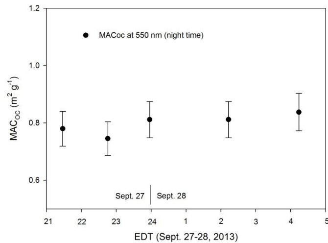
Figure R2. Mass absorption cross section (550nm) of wood smoke OC collected at night time (Sept. 27-28, 2013).
