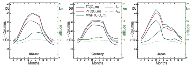
Figure 4: Validation and impact of \Delta on the pure tropospheric columns based on USeast, Germany and Japan seasonal cycles by comparing: \overline{\text{TC}}(\text{O}_3, m) , exactly what MOZAIC has measured in the troposphere (dark blue line); \overline{\text{PTC}}(\text{O}_3, m) , the MOZAIC pure tropospheric ozone column (red line); \overline{\text{MWPTC}}(\text{O}_3, m) , the composite MOZAIC-WOUDC tropospheric ozone column (blue line). All columns are expressed in DU. \Delta is the layer between z_{\text{top}} (dotted green line) and z_{\text{DT}} (solid green line), in km (right green vertical axis).
