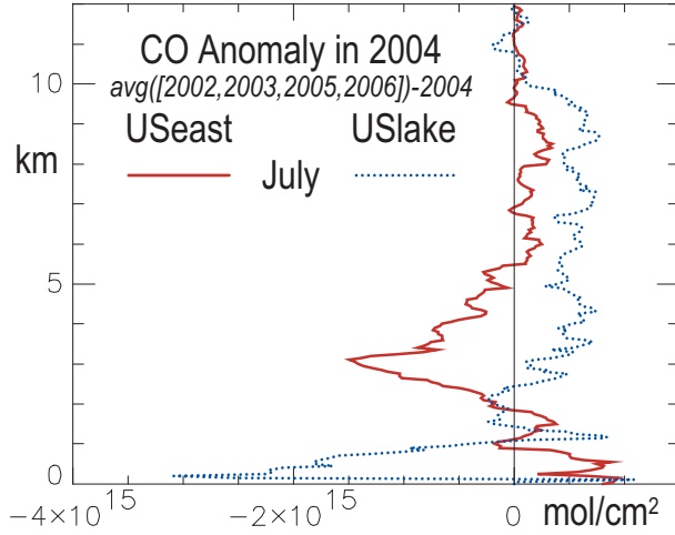
Figure S2: Monthly mean tropospheric profiles of the CO July 2004 anomaly (i.e. the average of (2002, 2003, 2005, 2006) minus 2004) at USeast (red line) and USlake (dotted blue line) in \text{mol}/\text{cm}^2 .
