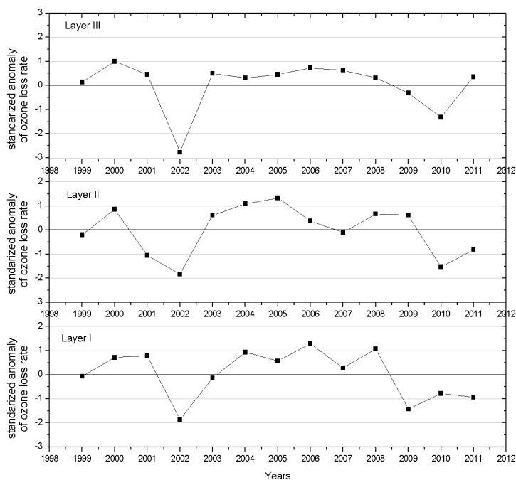
Fig. 1. Standardized anomalies of ozone loss rate
