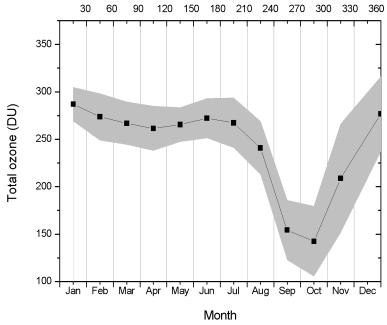
Fig. 2. Monthly mean total ozone column
