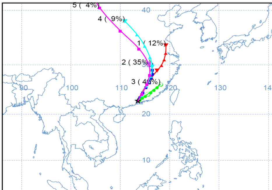
Fig. 6. Air mass clusters at WQS using HYSPLIT
