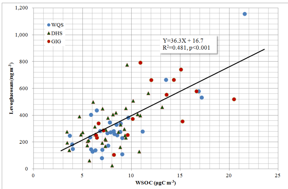
Fig. 4. Correlation between WSOC and levoglucosan
