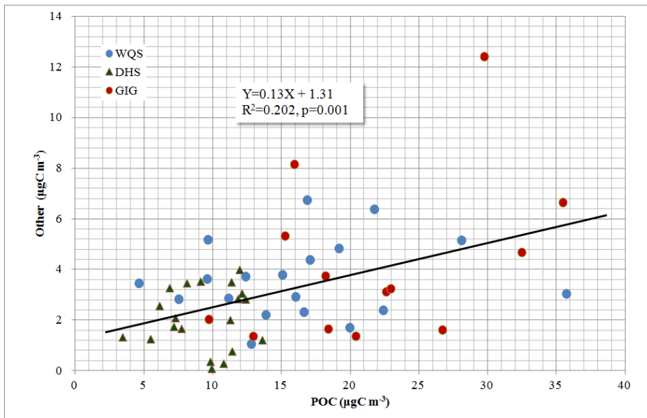
Fig. 3. Correlation between unexplained WSOC and POC
