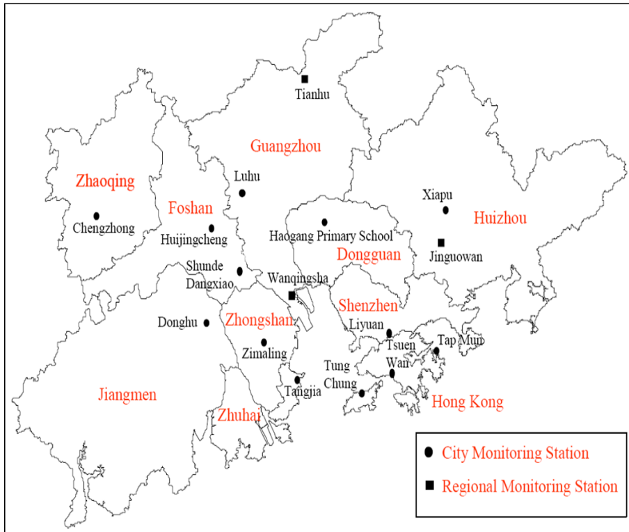
Fig. 5. PRD Regional Air Quality Monitoring Network
