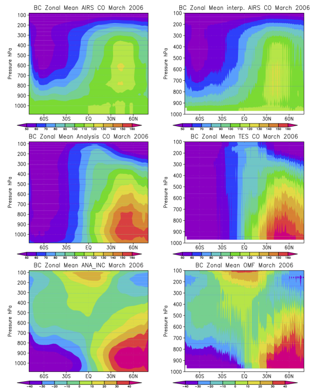
Fig. 3. Fig. 2b. As Fig. 2a, except with bias correction
