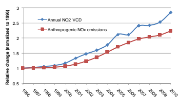
Figure 1 Inter-annual relative changes in the NO 2 VCD and anthropogenic NO x emissions. All data are normalized to the year 1996. Study region: 30°–40°N, and 110°–123°E. (Figure 12 in the revised manuscript)
