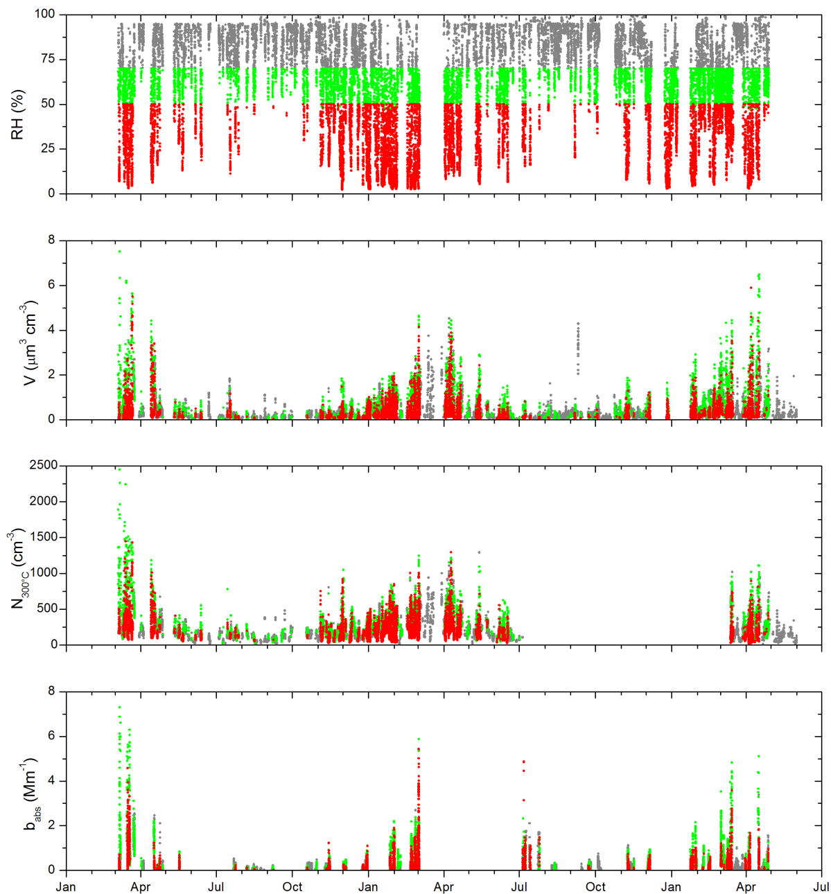
Figure 1: Time series of relative humidity RH (%), particle volume concentration V ( \mu\text{m}^3\text{cm}^{-3} ), refractory particle number concentration N_{300^\circ\text{C}} ( \text{cm}^{-3} ), and absorption coefficient b_{\text{obs}} ( \text{Mm}^{-1} ). The grey circles indicate data points selected for the LFT using local time and/or RH (see manuscript for further information). Green circles indicate observations at RH=0-70% and red circles indicate observations at RH 0-50%.
