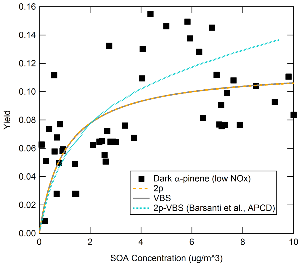
Fig. 2. Data from Fig. 3 in Barstanti et al. for low NO x dark alpha-pinene experiments, fit to 2p and VBS models over the range shown, and compared with the 2p-VBS best fit from Barsanti et al..
