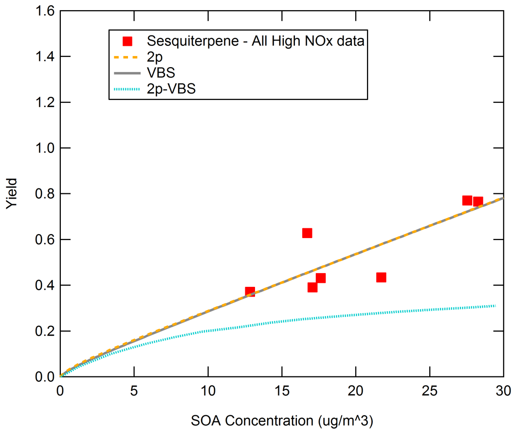
Fig. 3. Data from Fig. 4 in Barstanti et al. for high NOx sesquiterpene experiments, fit to 2p and VBS models over the range shown, and compared with the 2p-VBS best fit from Barsanti et al..
