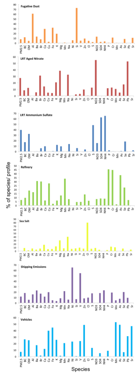
Fig. 1. Figure 8 Source profiles for the seven PMF factors
