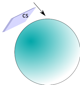
Figure 1: Schematic of an idealized contact nucleus approaching a supercooled droplet of water. (Not drawn to scale.) The surface labeled CS will have water adsorbed to it. In both Cooper's and Fukuta's proposed mechanisms, nucleation can be initiated anywhere on that surface which comes into contact with the droplet's surface. Therefore, both mechanisms predict a dependence on the size (i.e. surface area) of the contact nuclei.
