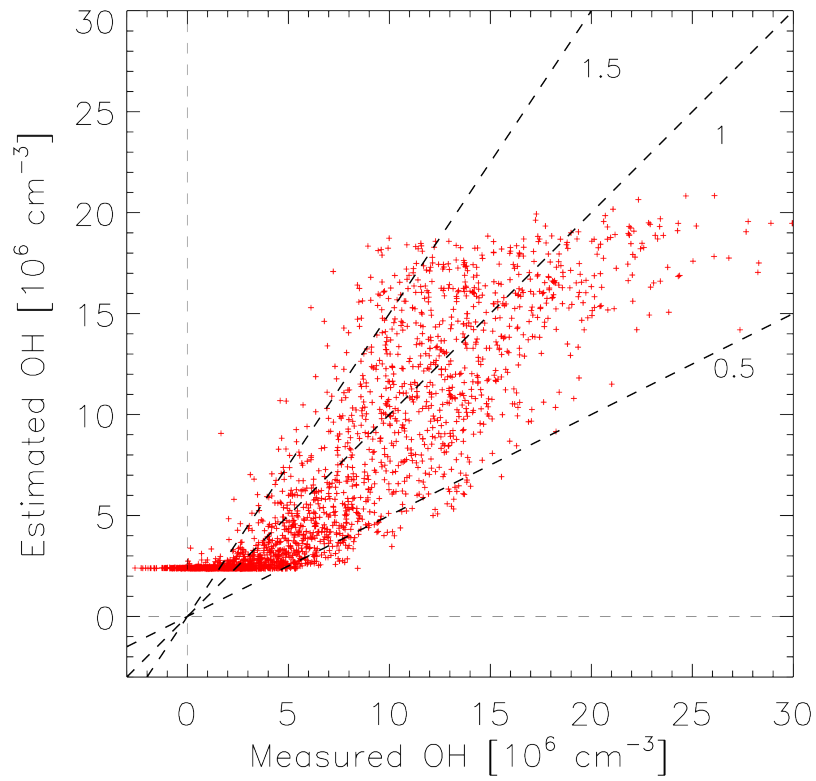
Fig. 1. Estimated OH concentration versus measured OH concentration during the PRD2006 campaign. The OH estimation was performed by using the empirical formula described by Lu et al. (2012).
