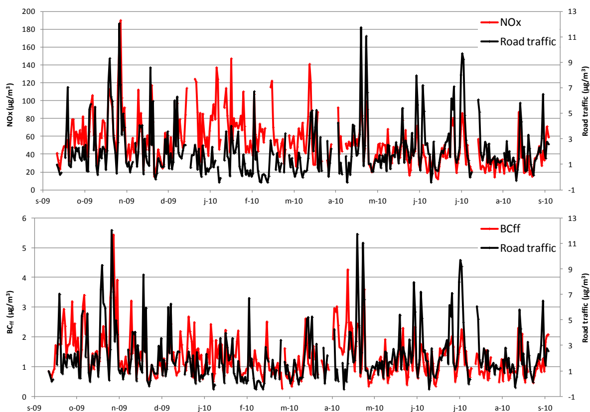
Fig. A.1.3.a. Comparison between the temporal variation of the PMF Road traffic factor and NOx (top) and BCff (bottom).
