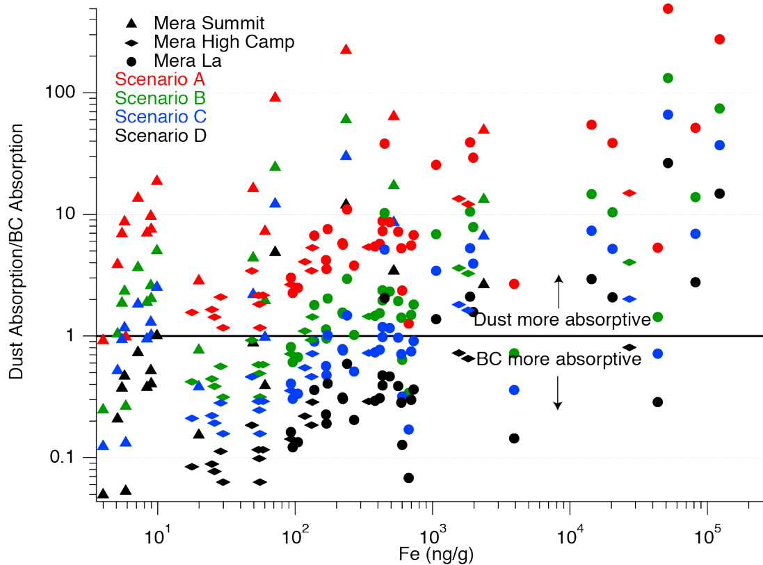
Fig. 2. Fe (ng/g) vs Dust Absorption/BC Absorption
