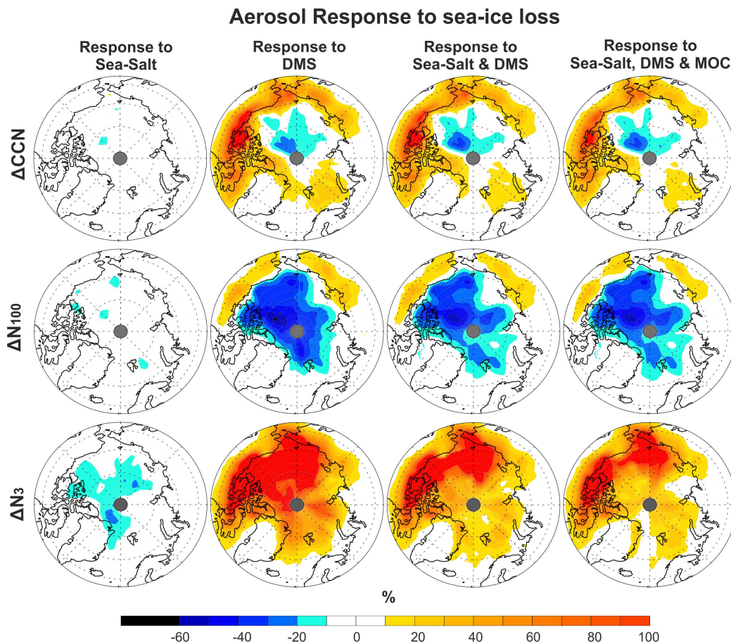
Fig. 1. Figure 4: aerosol response to sea-ice loss
