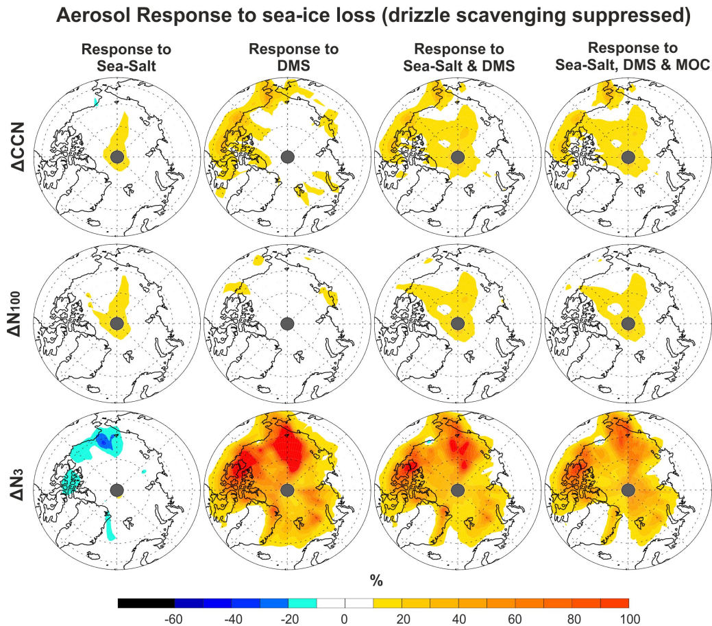
Fig. 2. Figure 5 (now 6): aerosol response to sea-ice loss (without drizzle)
