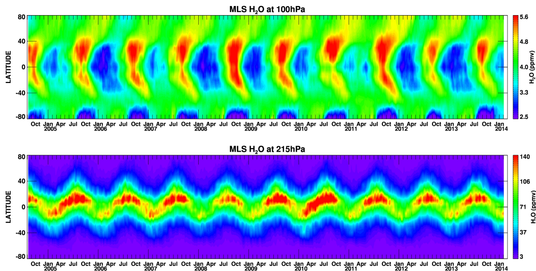
Fig. 1. Sample-Figure 1: Latitude-time sections of daily zonal-mean H 2 O at 100 and 215 hPa from MLS observation. Similar to Figure 4 in Jiang et al. (2010, JGR, doi:10.1029/2009JD013256)
