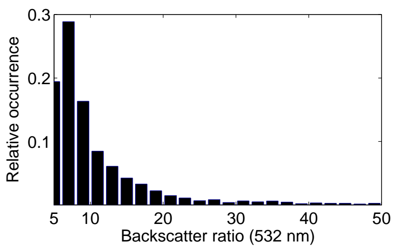
Fig. 2. Relative occurrences of CALIOP backscatter ratios for all measurements obtained during the 17 and 18 January 2010, which have been classified as ice according to Pitts et al. (2011).
