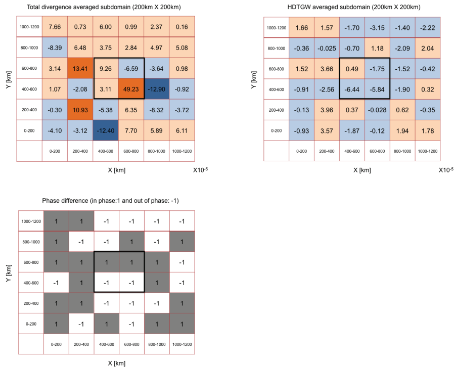
Fig. 2. Top left (right) shows total divergence (HDTGW) averaged over subdomain. Darker color shows the subdomain having larger value (over \pm 10 \times 10^{-5} ). Bottom figure shows same but phase differences.
