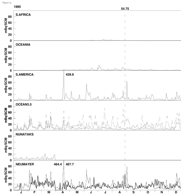
Fig. 1. STAG and AWI concentrations at Neumayer 1995
