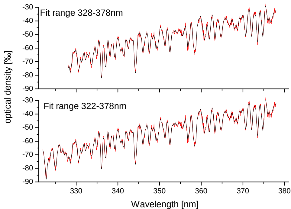
Fig. 1. Ring fit for the two different wavelength intervals (328–378 nm and 322–378nm)
