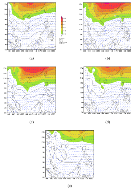
Figure 2. Climatological mean sea level pressure (contours; shaded for > 1016 hPa) superimposed with surface wind (in bars with contoured magnitude at 20 knots and more) at 00 UTC for (a) November, (b) December, (c) January, (d) February and (e) March.
