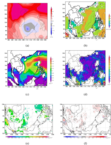
Figure 12. (a) Anomaly of mean sea level pressure (hPa), (b) average surface wave (vector with period (sec) shaded and height/swell (m) contoured), (c) average sea surface wind stress ( \text{Nm}^{-2} ), (d) average sea surface current ( \text{ms}^{-1} ), (e) average and (f) anomaly of chlorophyll-a concentration ( \text{mg}/\text{m}^3 ) during the period 16 – 20 January 2010.
