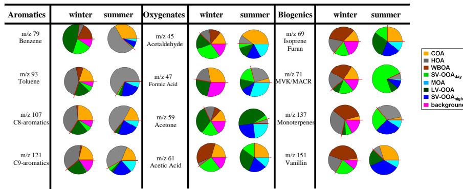
Fig. 9. VOCs source apportionment for selected aromatic, oxygenated and biogenic tracers. The solid red line defines the separation of the primary and secondary sources in the pie charts.
