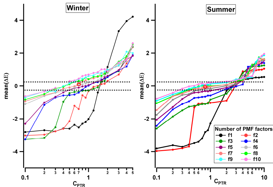
Fig. 1. \overline{\Delta E} values as function of the number of PMF factors (colors) and C_{PTR} for the winter and summer campaigns. PMF solutions within the dashed lines (corresponding to 25% deviation from \overline{\Delta E} equal to zero) were analyzed in detail. The selected wintertime solution has 6 factors and a C_{PTR} of 0.7, producing a \overline{\Delta E} value of -0.025 . The summertime solution has 7 factors and C_{PTR} of 0.8, producing a \overline{\Delta E} value of -0.053 . The chosen solutions are represented by the red circles.
