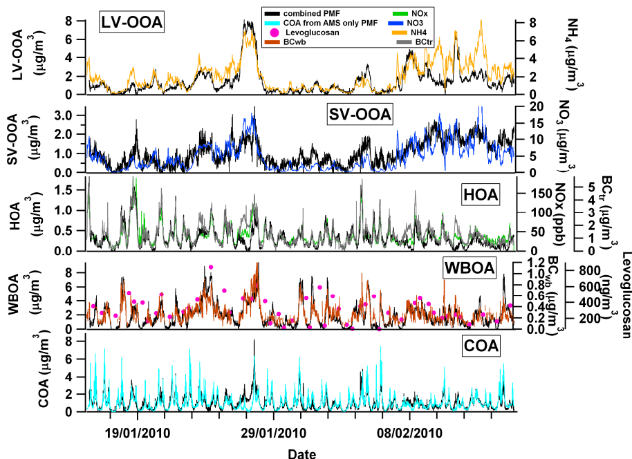
Fig. 3. Time series correlations between the retrieved PMF factors and external data (winter campaign). PMF factors concentrations are referred only to the AMS fraction. The PTR-MS factors have the same temporal variation as the AMS ones but different absolute and relative concentrations.
