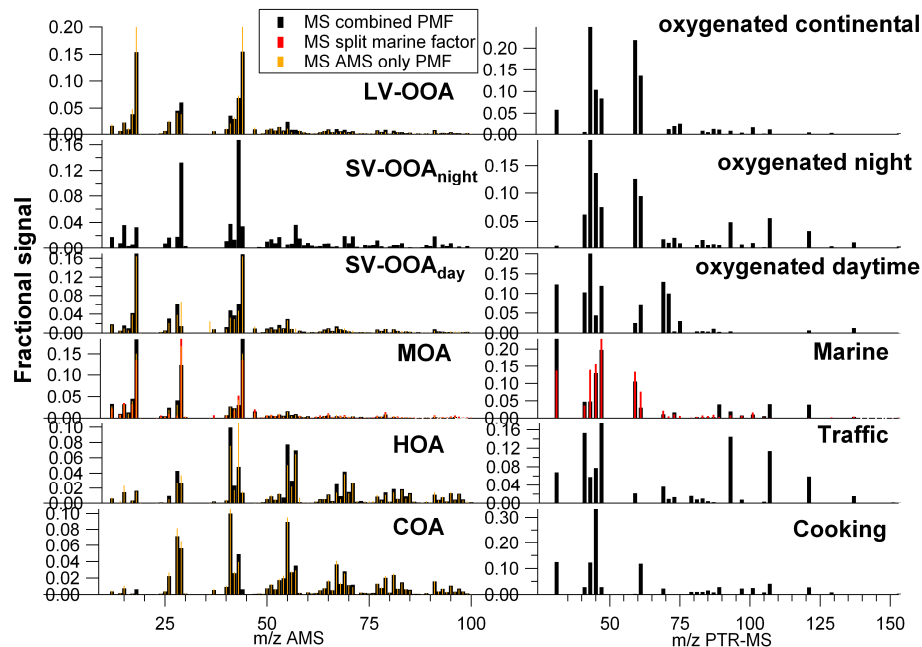
Fig. 5. Summertime AMS and PTR-MS source mass spectra separated with the combined PMF approach. The spectra comparison with the PMF AMS solution is also represented (Crippa et al., 2013b). In addition, in red the mass spectrum of the split marine factor from the 7-factor solution PMF is reported. Each mass spectrum is normalized to 1 both for the AMS and PTR-MS.
