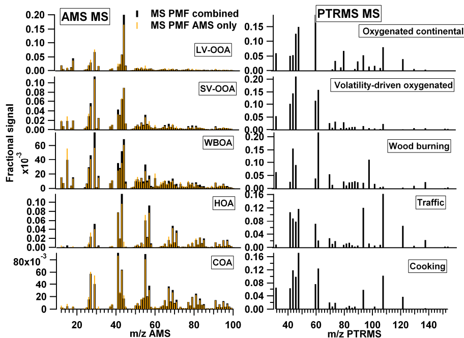
Fig. 2. Wintertime AMS and PTR-MS source mass spectra separated with the combined PMF approach. The spectra comparison with the \text{PMF}_{\text{AMS}} solution is also represented (Crippa et al., 2013a). Each mass spectrum is normalized to 1 both for the AMS and PTR-MS.
