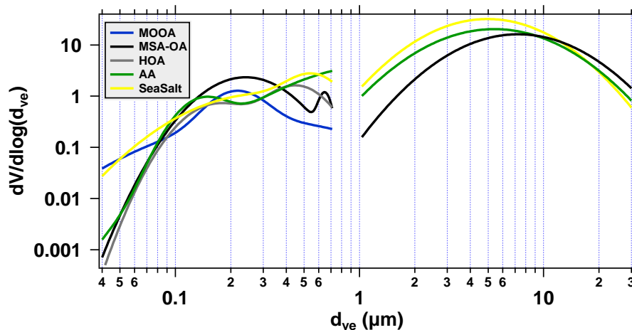
Fig. 7. Volume size distributions derived for individual PMF OA factors by the SMPS (a) and APS (b). The data was extracted from the time periods during which the respective factors dominated the submicron organic mass (> 66 %, and 50 % for sea salt), indicated by the red bars in Fig. 6b).
