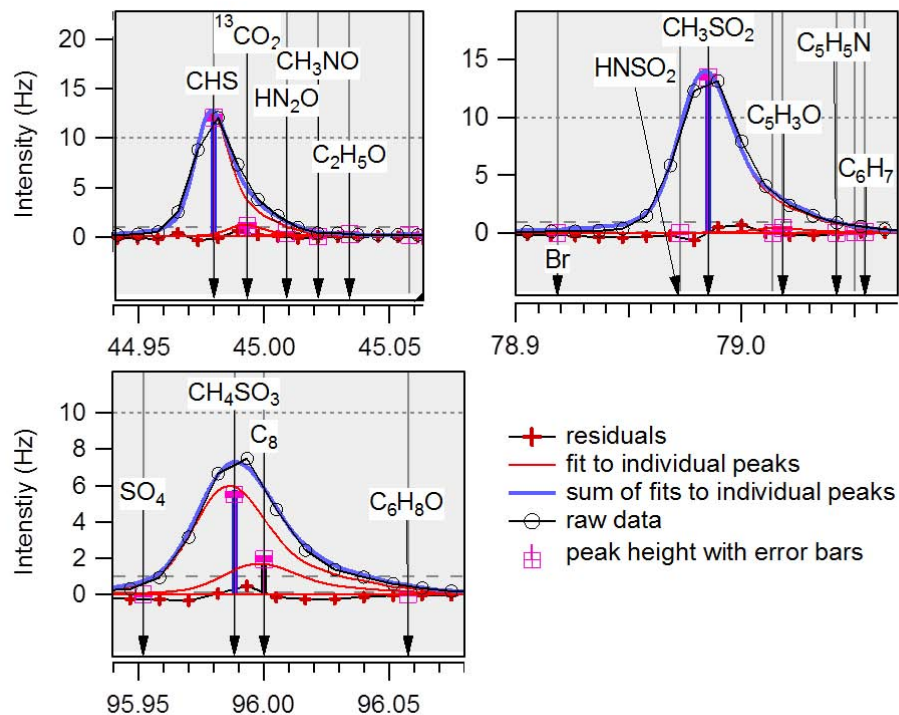
Fig. 9. Selection of high resolution marker ion fragment for methanesulfonic acid OA.
