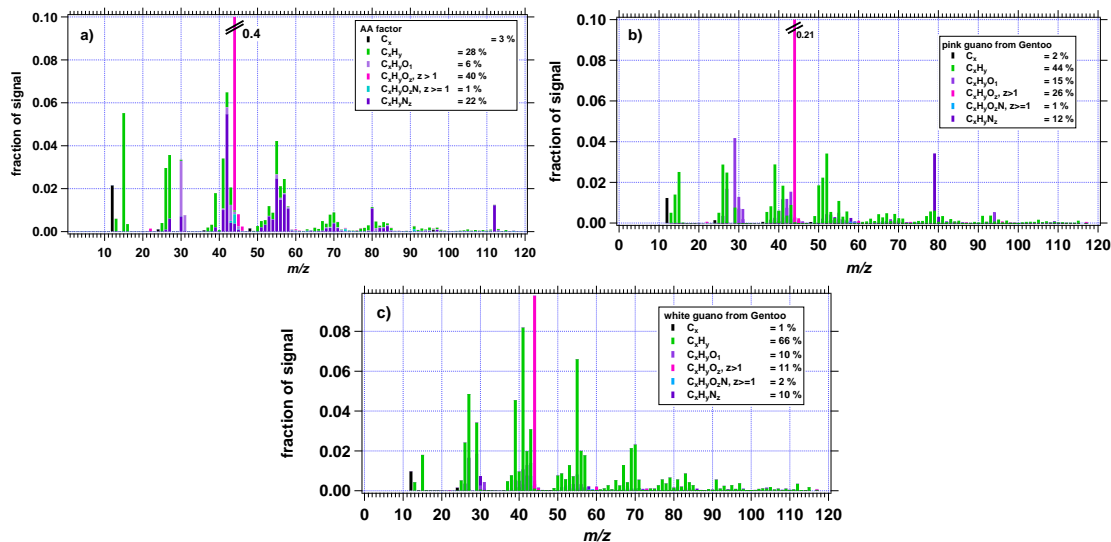
Fig. 13. Speciated organic mass spectrum of the amino acids/amines PMF factor (a) , pink guano from Gentoo (b) and white guano from Gentoo (c) . The percentages in the legend indicate the mass contribution to the total organic matter spectrum.
