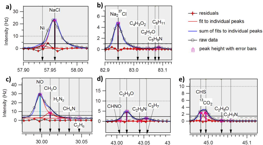
Fig. 10. HR ion fragment fits for two inorganic species and 3 organic species.
