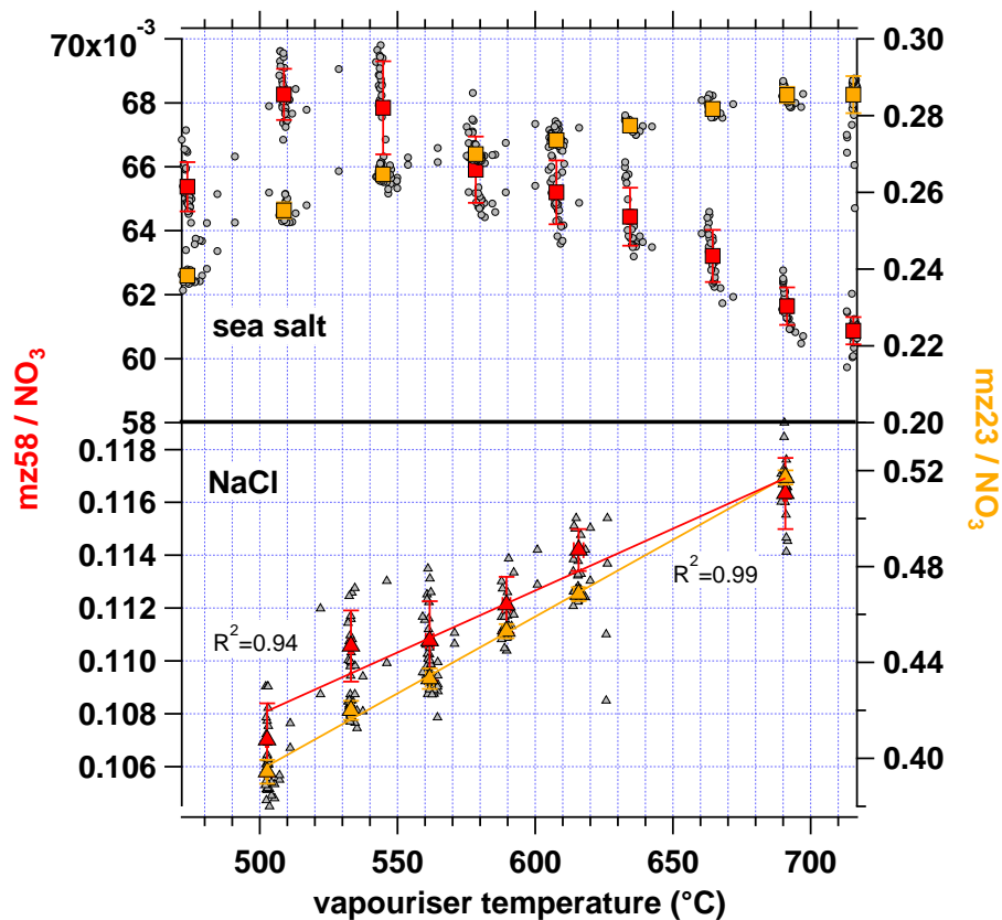
Fig. 2. Ratios of m/z 58 ( NaCl^+ ) and m/z 23 ( Na^+ ) over particulate nitrate for a solution of standard sea salt (SIGMA-Aldrich S9883, upper panel) with ammonium nitrate (mass ratio 0.9) and for a solution of pure NaCl (lower panel) with ammonium nitrate (mass ratio 1.1) as function of vapouriser temperature.
