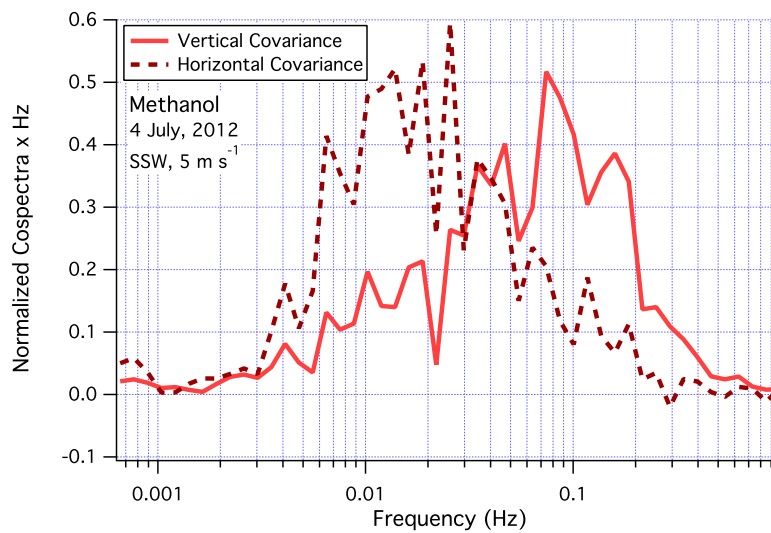
Fig. 14. Normalized methanol cospectra for vertical covariance (same as Fig. 5) and horizontal covariance on 4 July. The horizontal cospectrum peaked at a lower frequency than the vertical cospectrum, likely related to spatial inhomogeneity.
