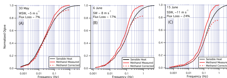
Fig. 7. Ogives of sensible heat and methanol (before and after attenuation correction) for three days of different wind speeds and atmospheric stability. Flux loss at high frequencies increased with wind speed and stability, where a greater contribution to the flux came from smaller eddies.
