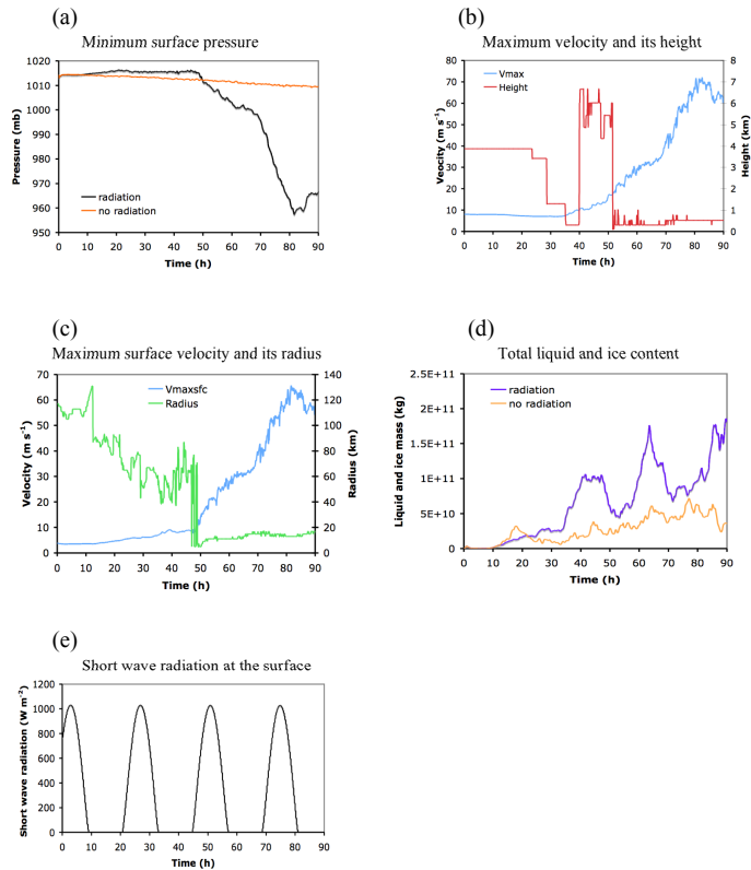
Fig. 10. Time series for Experiment 15. (a) Minimum surface pressure, including comparison with the non-radiation case. (b) The azimuthally averaged maximum tangential velocity and the height it occurs. (c) The azimuthally averaged tangential velocity at the lowest model level and the radius it occurs. (d) Total liquid and ice mass content in a cylindrical volume of radius 100 km from the center. (e) Clear sky short wave radiation at the surface.
