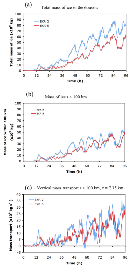
Fig. 12. Comparison of Experiments 2 and 5. (a) The total mass of ice in the fine grid domain. (b) The total mass of ice within a radius of 100 km of the center of the domain. (c) The vertical mass transport of air within a radius of 100 km of the center of the domain, at z = 7.35 km.
