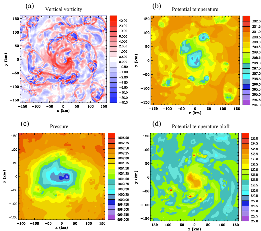
Fig. 14. Horizontal sections for Experiment 2, at t = 78 h. (a) Vertical vorticity ( \times 10^{-4} \text{rads}^{-1} ), (b) potential temperature (K), (c) pressure (mb), at z = 98 m, and (d) potential temperature (K), at z = 7.35 km.
