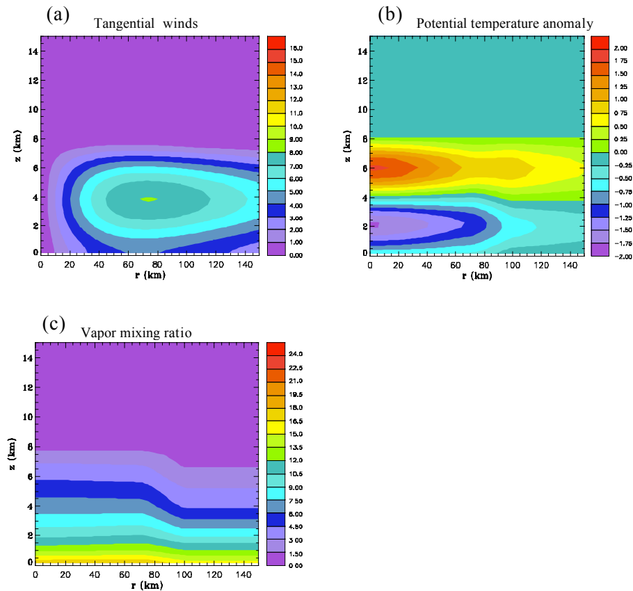
Fig. 1. Initial conditions for a small weak vortex with a moisture anomaly. (a) Tangential winds. The contour interval is 1 \text{ ms}^{-1} . (b) Potential temperature anomaly. The contour interval is 0.25 \text{ K} . (c) Water vapor mixing ratio. The contour interval is 1.5 \text{ g kg}^{-1} .
