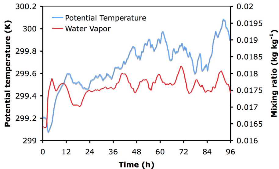
Fig. 16. Time series of the average potential temperature and water vapor mixing ratio within 100 km of the center, at z = 305 m, for Experiment 2.
