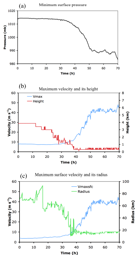
Fig. 2. Time series for Experiment 1, the no ice case. (a) The minimum surface pressure. (b) The azimuthally averaged maximum tangential velocity and the height it occurs. (c) The azimuthally averaged tangential velocity at the lowest model level and the radius it occurs.
