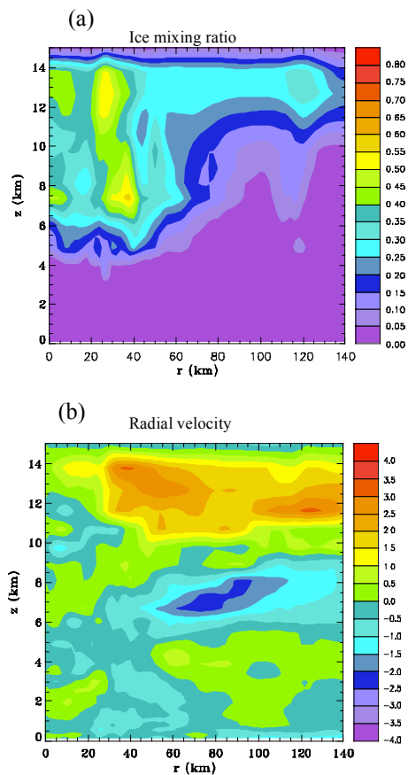
Fig. 11. Azimuthally averaged fields of (a) Mixing ratio of ice ( \text{g kg}^{-1} ), and (b) radial component of wind velocity ( \text{m s}^{-1} ), at t = 75 h, for Experiment 2.
