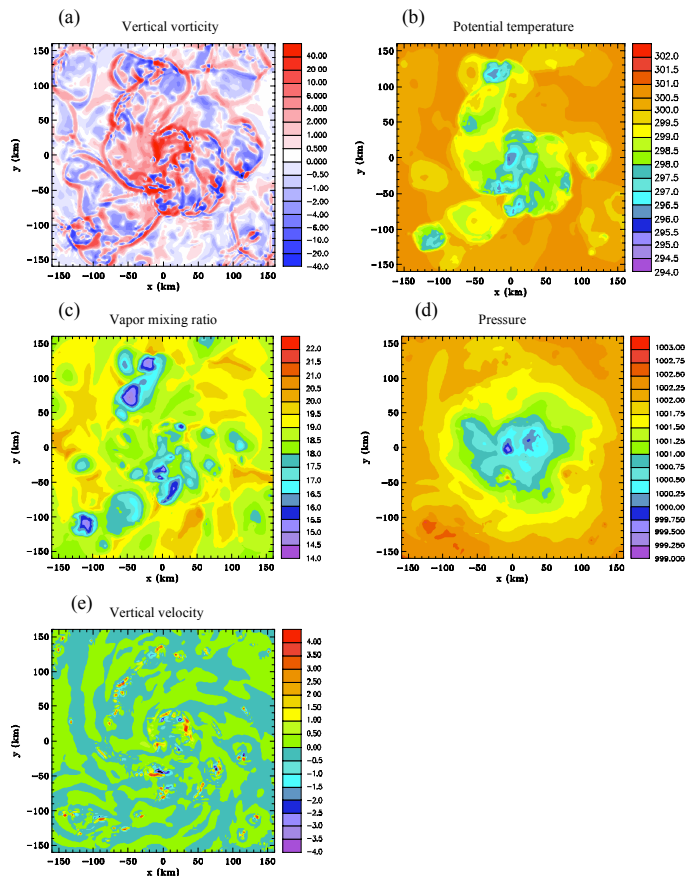
Fig. 15. Horizontal sections for Experiment 2, at t = 80\text{h} . (a) Vertical vorticity ( \times 10^{-4}\text{ rad s}^{-1} ), (b) potential temperature (K), (c) water vapor mixing ratio ( \text{g kg}^{-1} ), (d) pressure (mb), at z = 98\text{m} , and (e) vertical velocity ( \text{m s}^{-1} ), at z = 1.6\text{km} .
