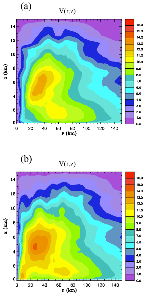
Fig. 4. Azimuthally averaged tangential velocity V(r,z) for Experiment 2, at (a) t = 79 h, and (b) t = 83 h. The contour interval is 1 \text{ m s}^{-1} .
