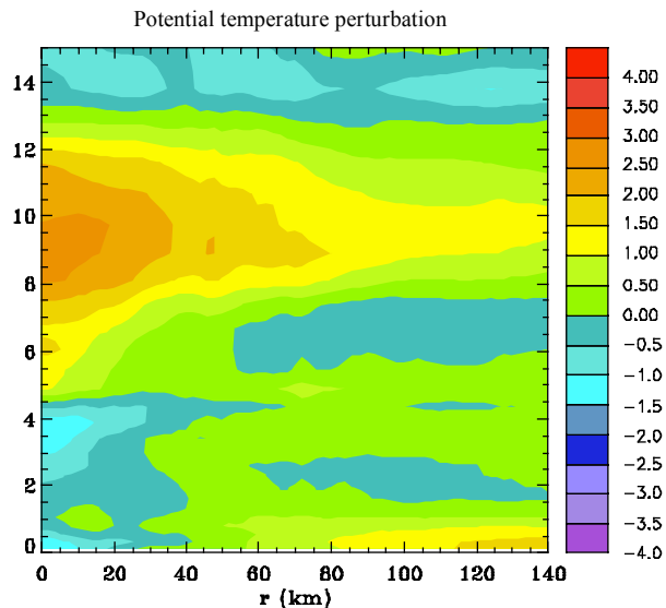
Fig. 13. The azimuthally averaged potential temperature perturbation for Experiment 2, at t = 79 h. The contour interval is 0.5 K.
