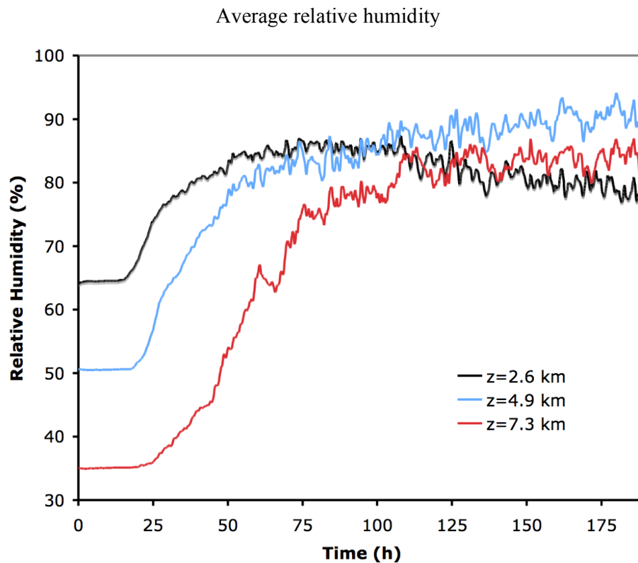
Fig. 6. The average relative humidity for a circular area with radius of 100 km from the vortex center, at levels z = 2.6, 4.9 and 7.3 km, for Experiment 3.
