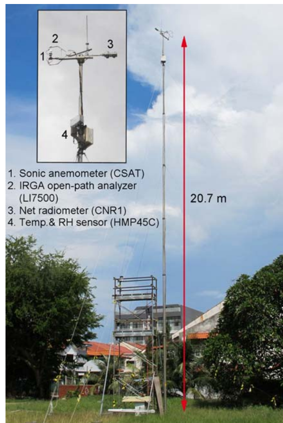
Figure S3. Photograph of the flux tower and EC system (inset). The azimuth orientation of the sonic anemometer corresponds to the main wind direction of the prevailing monsoon season ( 180^\circ or 30^\circ ).
