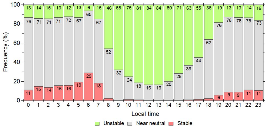
Figure S6. Frequency distribution of atmospheric stability during the entire measurement period. Numbers inside bars indicate percentage of periods for each stability condition defined in Fig. S4.
