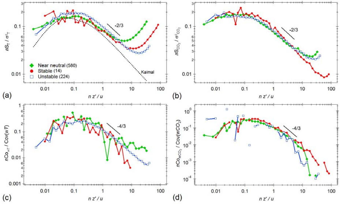
Figure S4. Composite (co)spectra of (a) virtual temperature (b) \text{CO}_2 , and fluxes of (c) sensible heat and (d) \text{CO}_2 , for three stability ranges (unstable: z'/L < -0.1 , near neutral: -0.1 \leq z'/L < 0.1 , and stable: z'/L \geq 0.1 . L is Obukhov length and z' is effective measurement height ( z' = z_m - z_d )). Results are based on 818 30-min periods with at least 17,700 10 Hz data points each, measured between 2-22 February 2012. Numbers in parenthesis in (a) are number of periods for each stability category. The (co)spectral energy densities are normalized by their respective (co)variance and plotted as a function of a non-dimensional frequency where n is natural frequency and u is mean horizontal wind speed. The dashed line in (a) represents a neutral reference spectra for a flat, ideal surface (Kaimal et al. 1972).
