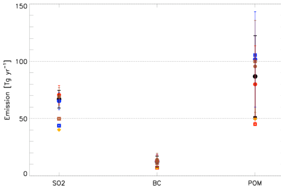
Fig. 10. Global yearly FG (squares) and AN (circles) emissions of \text{SO}_2 , BC and POM from experiment ACFED (black), ACFAS (blue), AEFED (red) and AEFAS (brown) for the year 2010. Vertical lines correspond to uncertainties of the corresponding fluxes. Projected RCP emissions are also illustrated (diamond gold).
