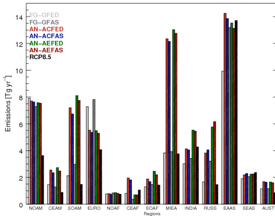
Fig. 7. Annual FG and AN SO 2 emissions for all four combinations of anthropogenic emissions inventories (ACFED, ACFAS, AEFED and AEFAS) for regions illustrated in Fig. 1a.
