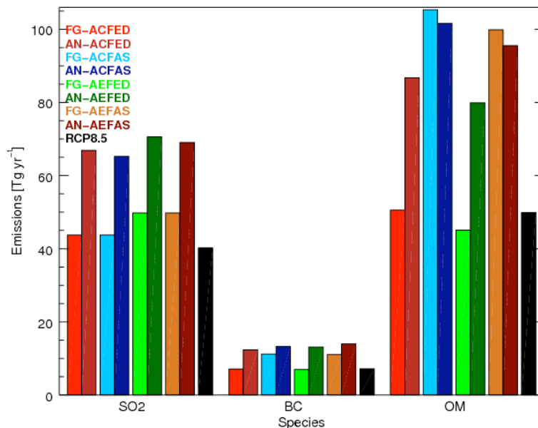
Fig. 6. Same as Fig. 3 but for all four combinations of anthropogenic and biomass burning emission inventories: ACFED, ACFAS, AEFED and AEFAS.
