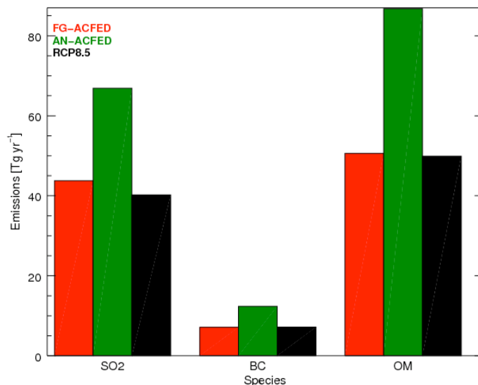
Fig. 3. Global yearly emissions of \text{SO}_2 (in \text{Tg yr}^{-1} ), BC and POM (in \text{Tg yr}^{-1} ) of first guess (FG, red), analysis (AN, green) and projected RCP8.5 emissions for the year 2010 (RCP, black). The FG combines the anthropogenic emissions from L10 and the GFED biomass burning emissions.
