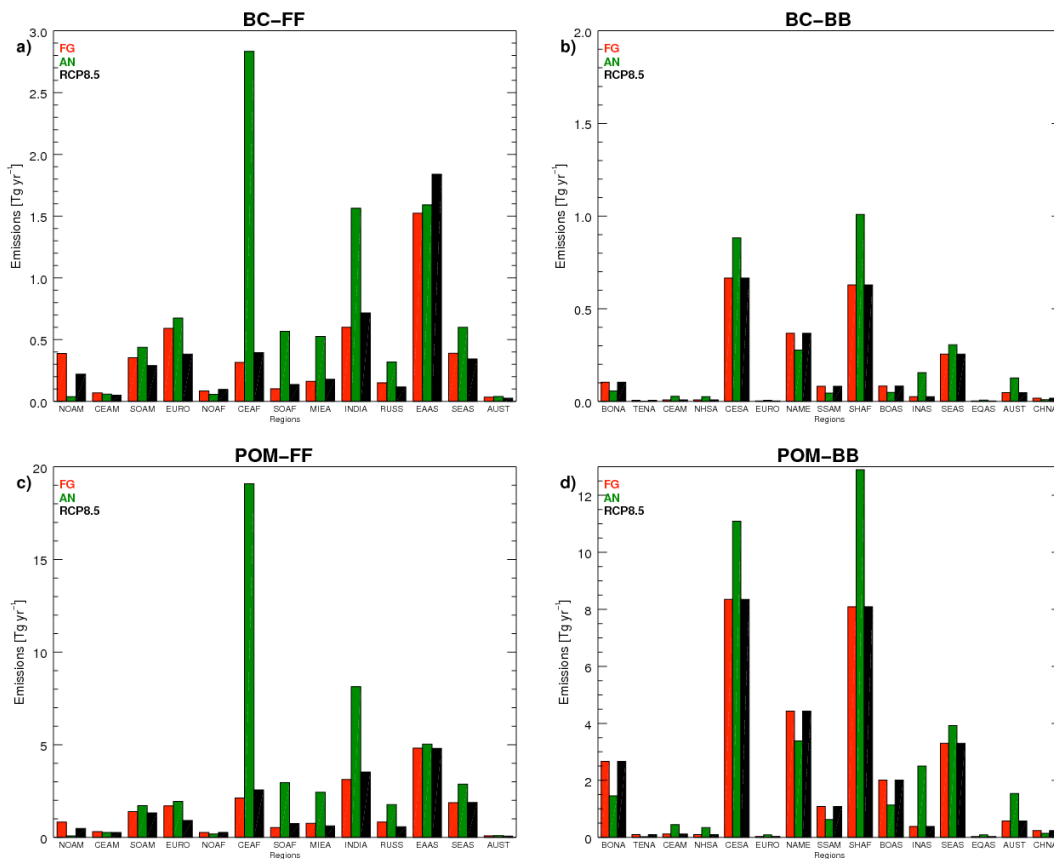
Fig. 5. Same as Fig. 3 but for annual emissions of (a) BC and (c) POM from fossil fuel combustion in the thirteen regions illustrated in Fig. 1a and annual emissions of (b) BC and (d) POM from biomass burning in the fifteen regions illustrated in Fig. 1b.
