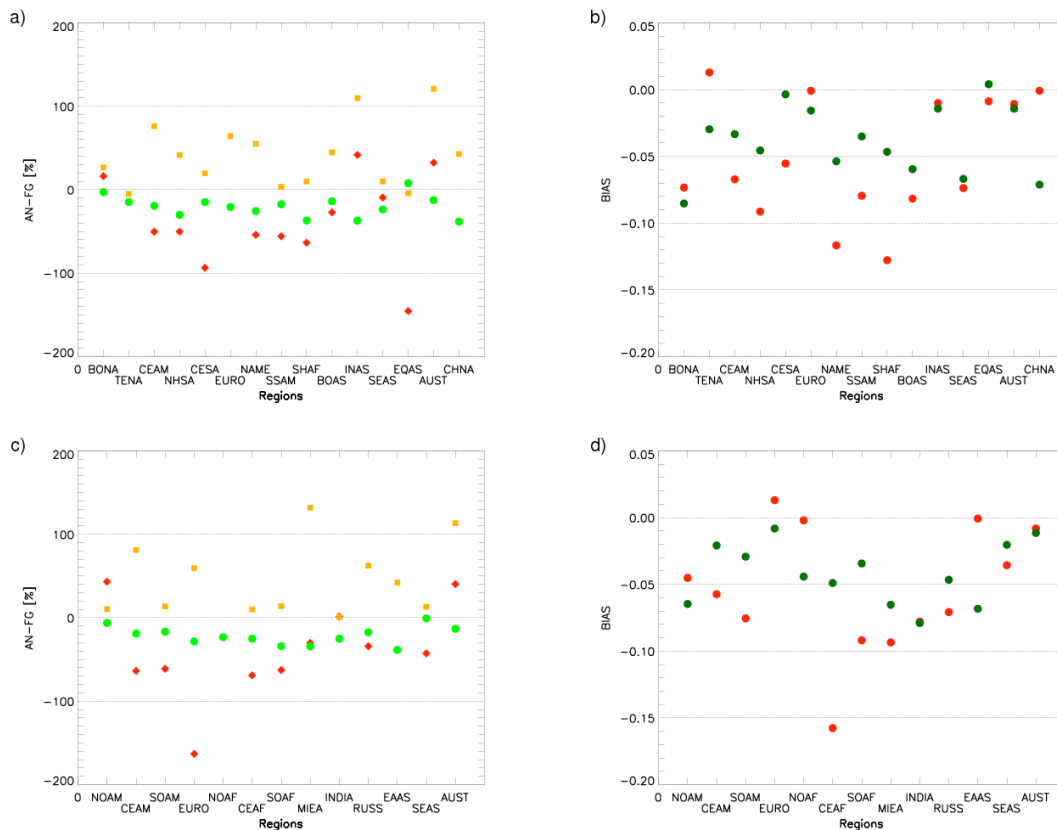
Fig. 2. Total AOD change in rms error (green circles), mean bias (red diamond) and correlation (orange squares) between FG and AN with respect to MODIS AOD for (a) biomass burning and (c) industrial regions. In addition, bias for FG (red) and AN (green) with respect to MODIS for (b) biomass burning and (d) industrial regions are illustrated.
