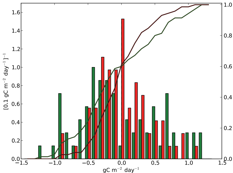
Fig. 4. Normalized distribution (bars, left axis) and cumulative distribution function (lines, right axis) of the monthly misfits in NEE ( \text{gCm}^{-2} \text{day}^{-1} ) between ORCHIDEE (green) or the inverted NEE (red) and the CE-L4 averages from Fig. 2.
