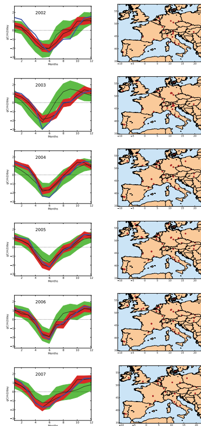
Fig. 2. Temporal evolution of monthly (i.e. 30-day mean) NEE ( \text{gCm}^{-2}\text{day}^{-1} ; negative values: sink) at the CE-L4 locations specified for a full year in the maps. Blue: CE-L4 data averages; green: ORCHIDEE; red: inverted fluxes; shaded areas: NEE \pm standard deviation of the uncertainty in NEE.
