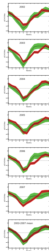
Fig. 3. Temporal evolution of monthly (i.e. 30-day mean) NEE ( \text{gCm}^{-2}\text{day}^{-1} ; negative values: sink) over the whole European domain of CHIMERE. Green: ORCHIDEE; red: inverted fluxes; shaded areas: NEE \pm standard deviation of the uncertainty in NEE. Dotted lines: NEE \pm standard deviation of the variations of NEE for a given month from 2002 to 2007.
